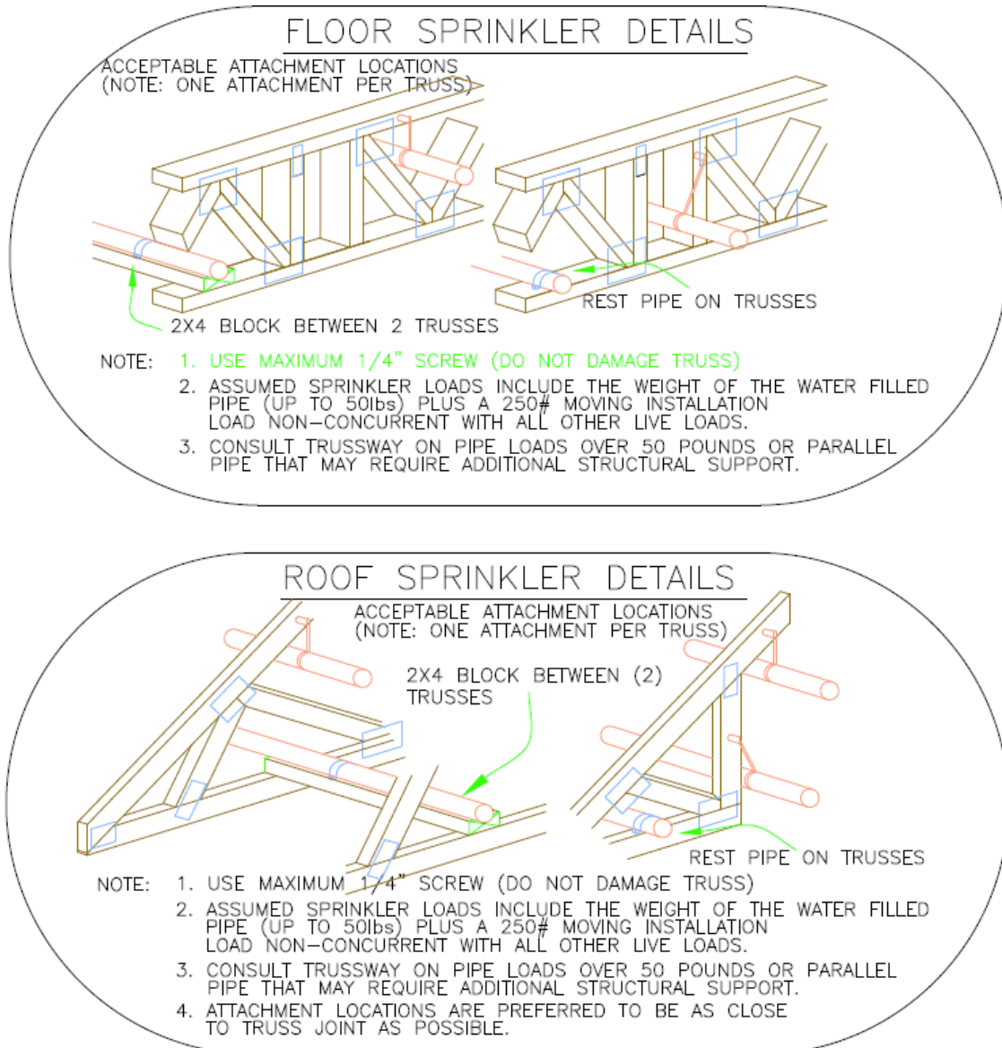
Figure 1: Assumed Sprinkler Attachments to Trussway Trusses
