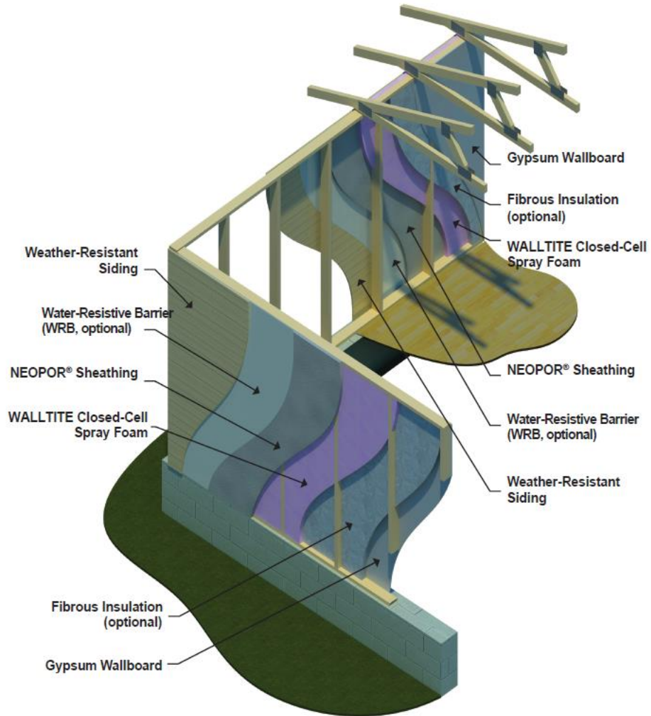
Figure 1a: Illustration of BASF HP+ Wall E Series
