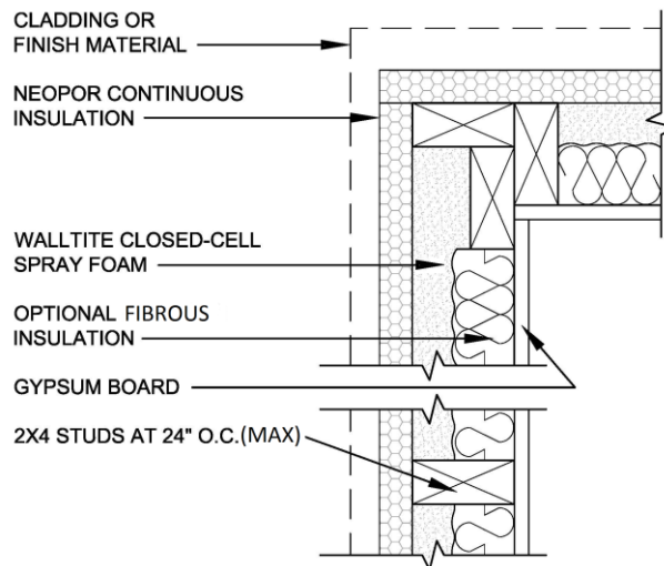
Figure 1b: Cross Section of BASF HP+ Wall E Series Layers
