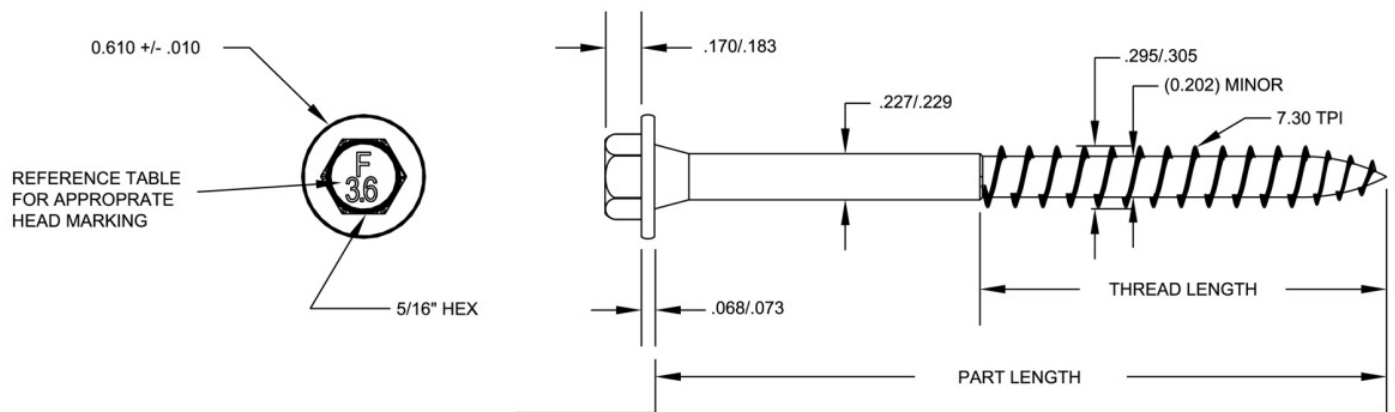
Figure 1. LedgerLOK® Ledger Board Fasteners (in)
