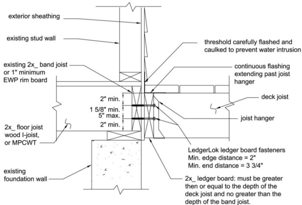
Figure 2. LedgerLOK® Ledger Board Fastener Deck Connection
