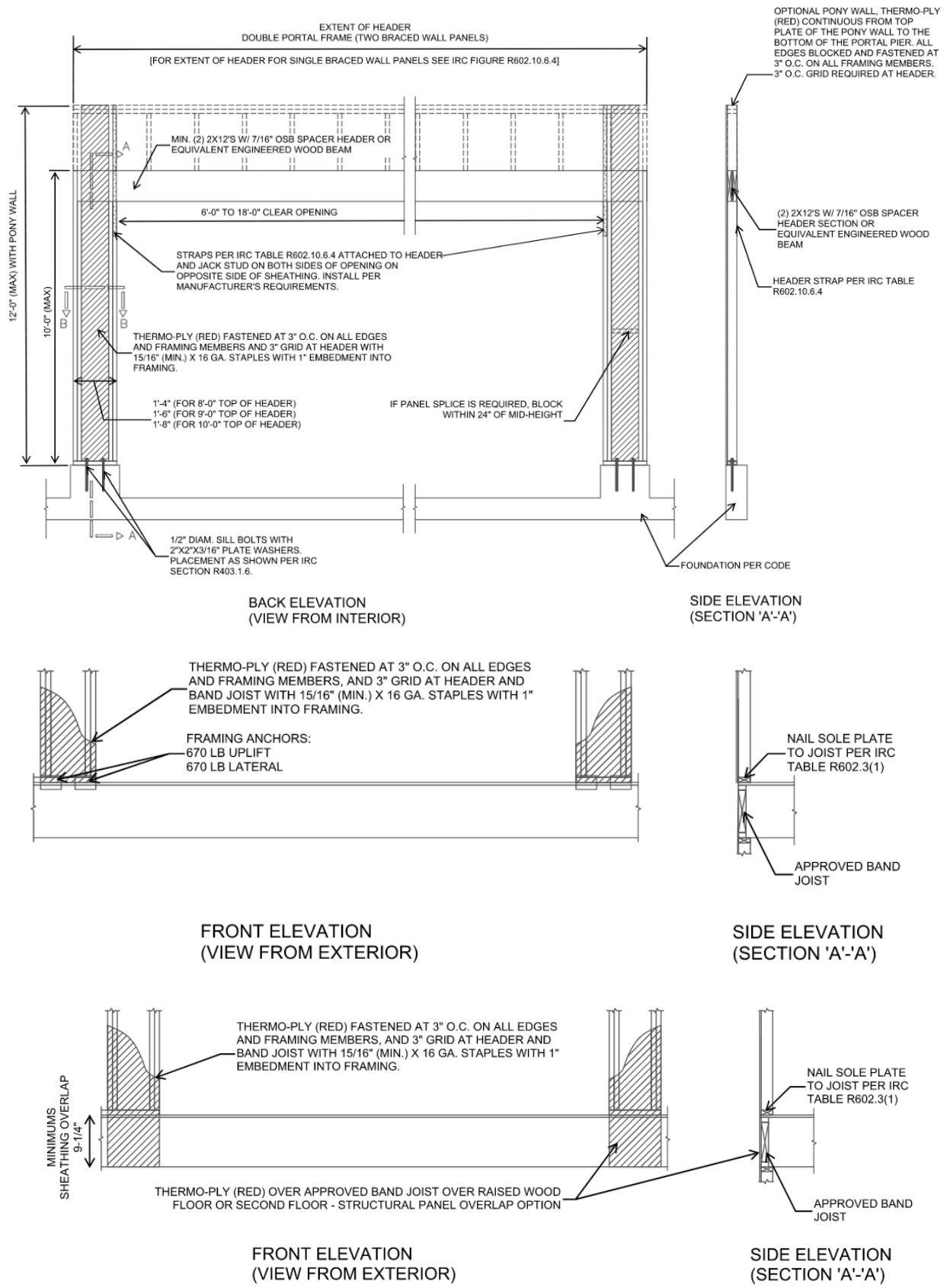
Figure 2. Thermo-Ply® Red Structural Sheathing CS-PF
