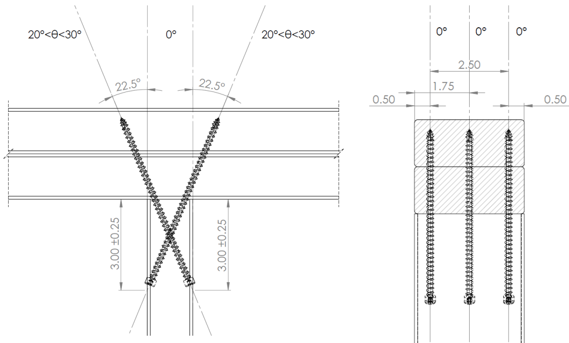
Figure 8. Stud to Top Plate – 22.5° (Angle), Three Fastener Install Option
