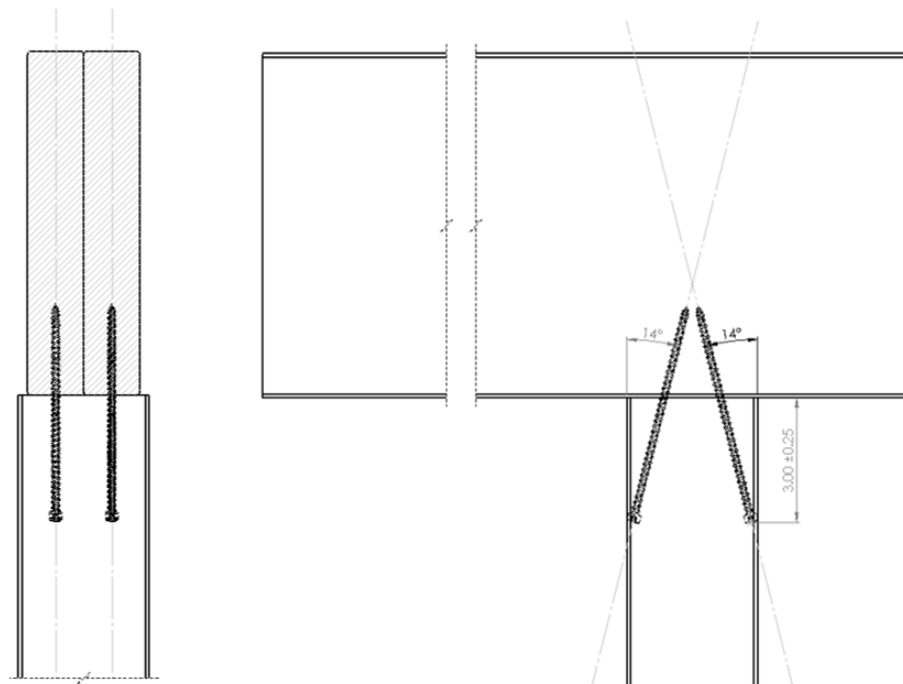
Figure 17. Post to Beam - Deck Connection
