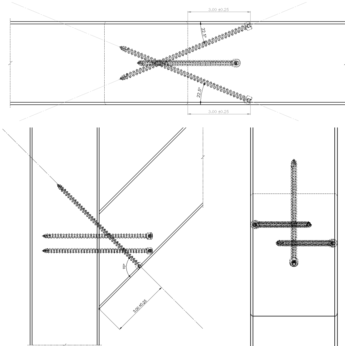
Figure 21. 4 x 4 Diagonal Brace Connection using CAMO Truss Screws
