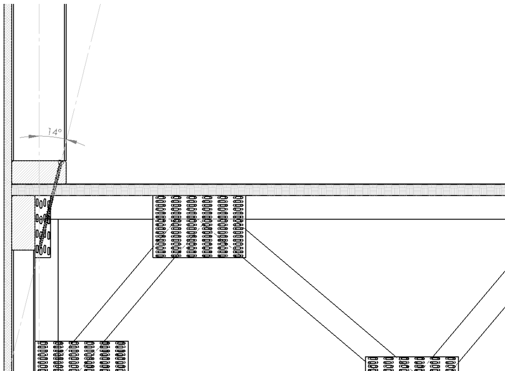
Figure 5. Installation of Fasteners at an Angle in Bottom Plate to Floor Truss/Joist Applications
