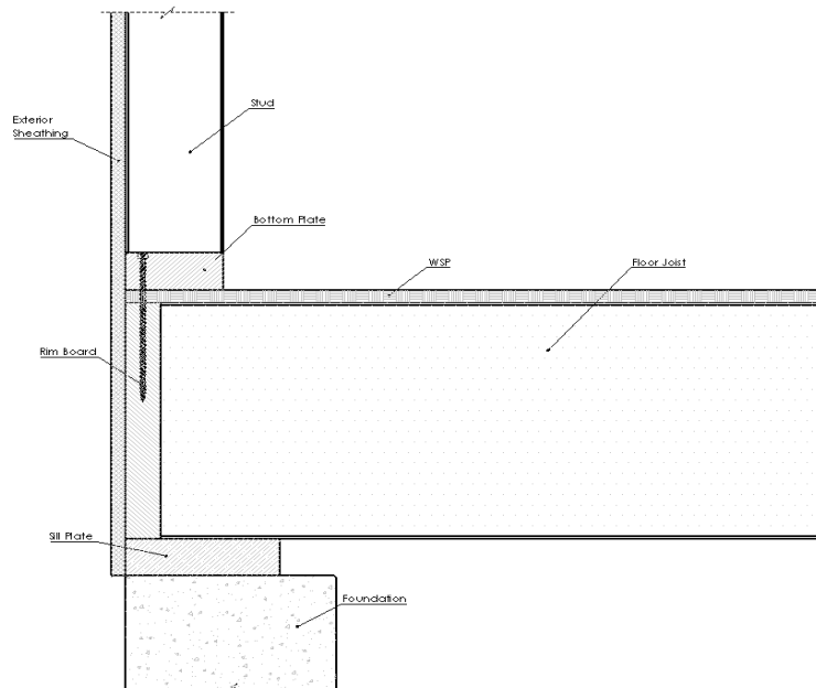
Figure 15. Fastener in Bottom Plate to Rim Board Connection
