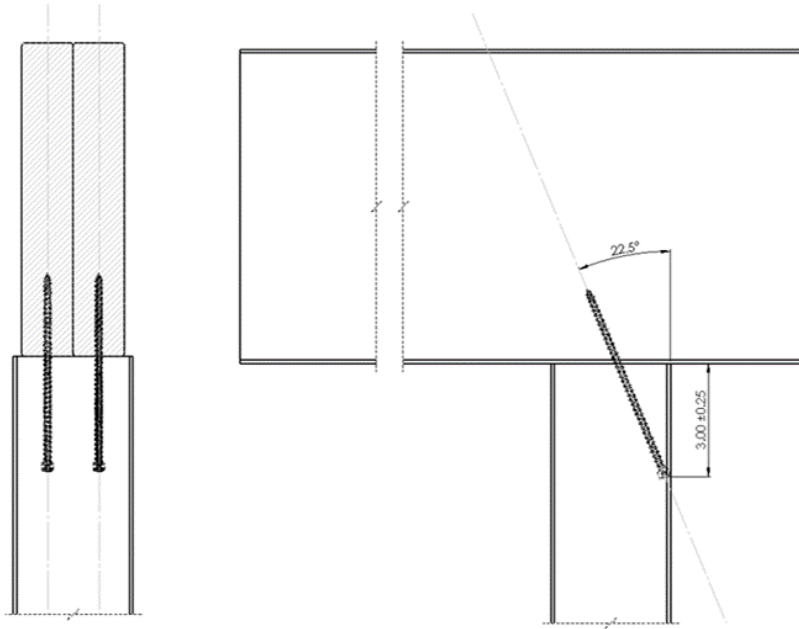
Figure 18. Post to Beam - Deck Connection
