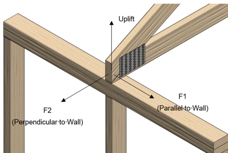
Figure 2. Uplift and Lateral Load Orientations
