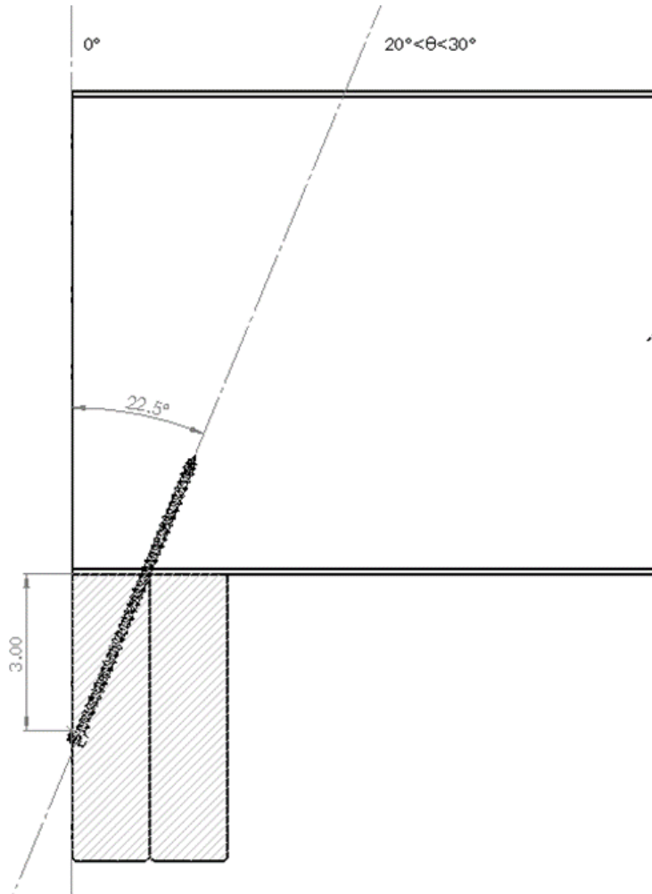
Figure 16. Joist to Beam - Deck Connection
