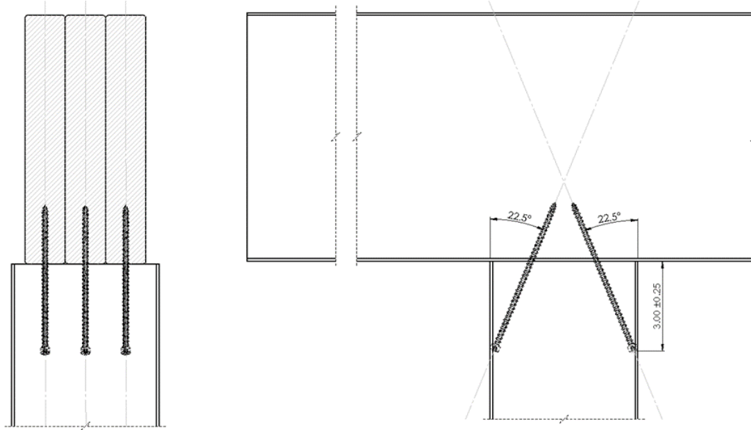
Figure 20. Post to Beam - Deck Connection
