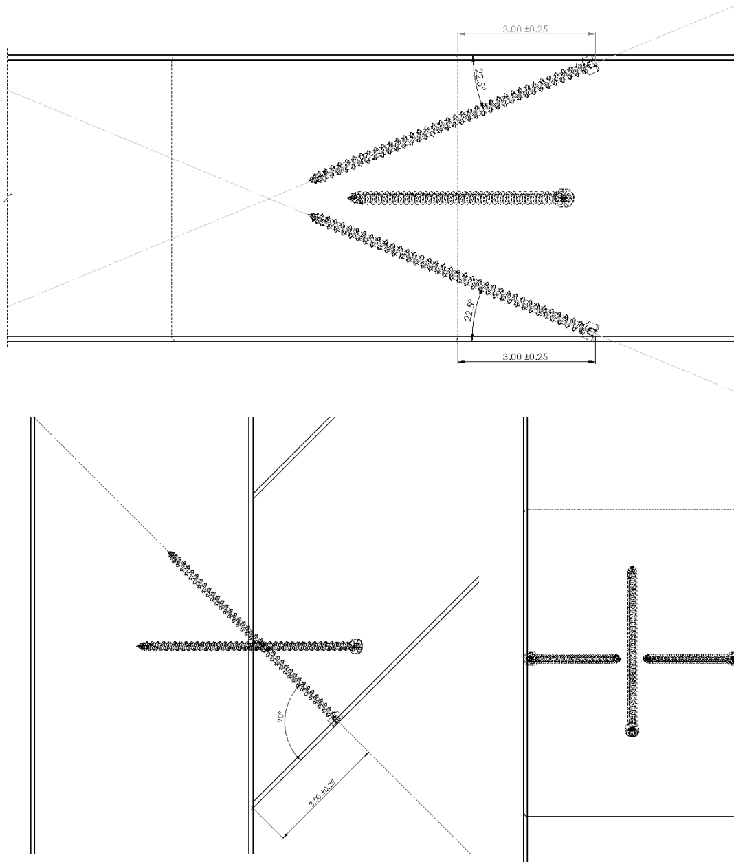
Figure 22. 6 x 6 Diagonal Brace Connection using CAMO Truss Screws
