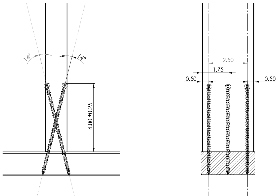
Figure 13. Stud to Bottom Plate – 4°-14° (Angle), Three Fastener Install Option
