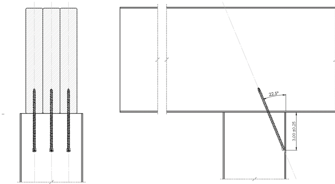
Figure 19. Post to Beam - Deck Connection
