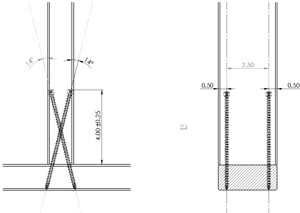
Figure 12. Stud to Bottom Plate – 4°-14° (Angle), Two Fastener Install Option
