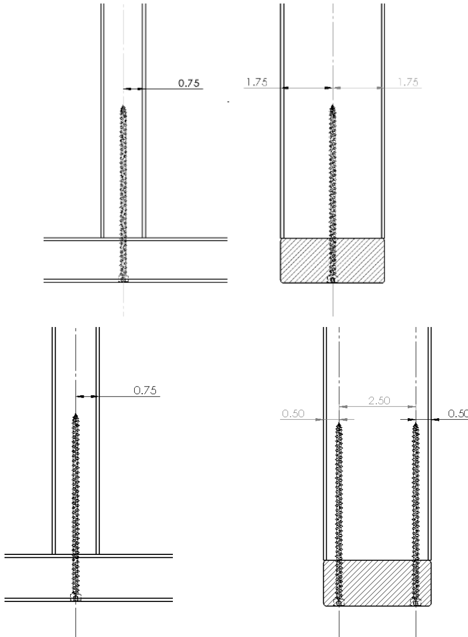
Figure 14. Stud to Bottom Plate – 0° (Perpendicular) Install Options
