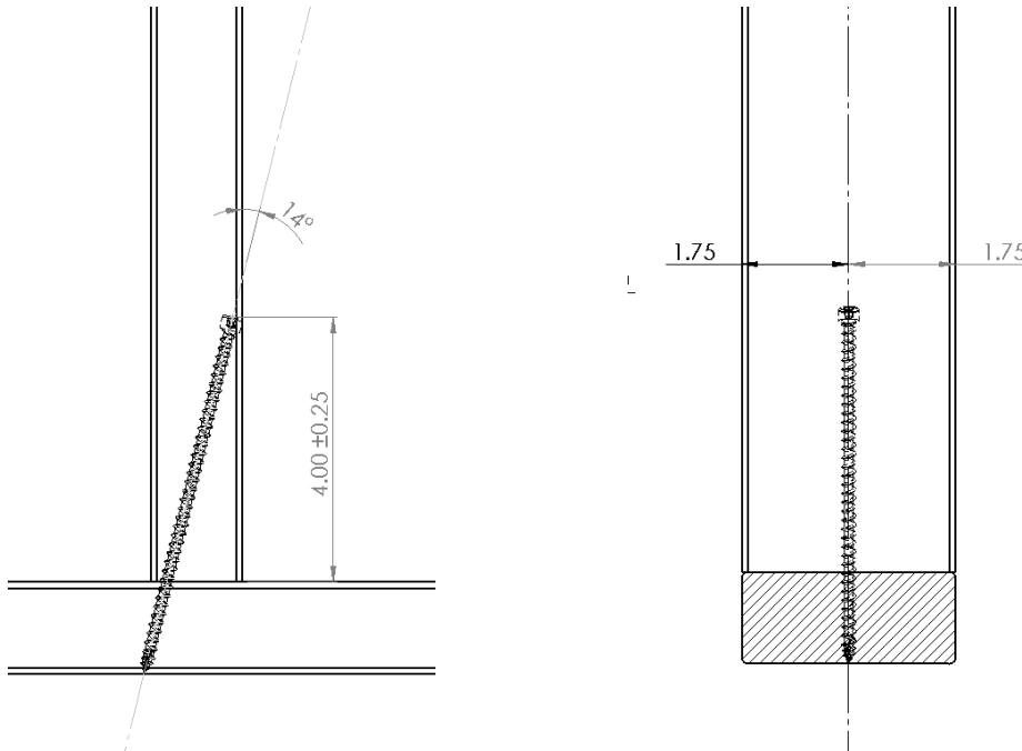
Figure 11. Stud to Bottom Plate – 14° (Angle), One Fastener Options
