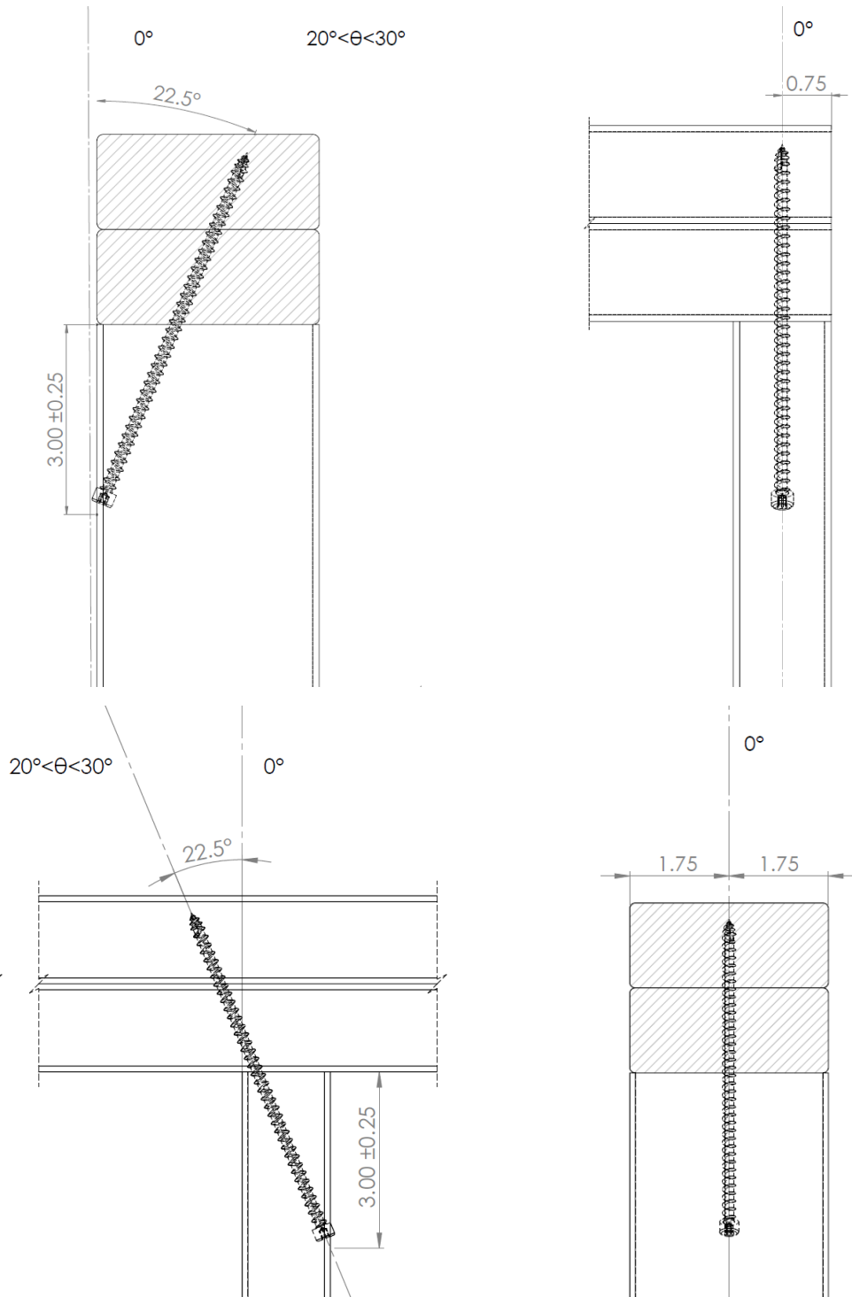
Figure 6. Stud to Top Plate – 22.5° (Angle), One Fastener Options
