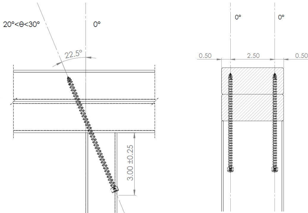
Figure 7. Stud to Top Plate – 22.5° (Angle), Two Fastener Install Option
