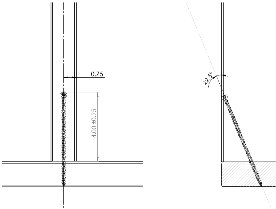
Figure 10. Stud to Bottom Plate – 22.5° (Angle), One Fastener Options
