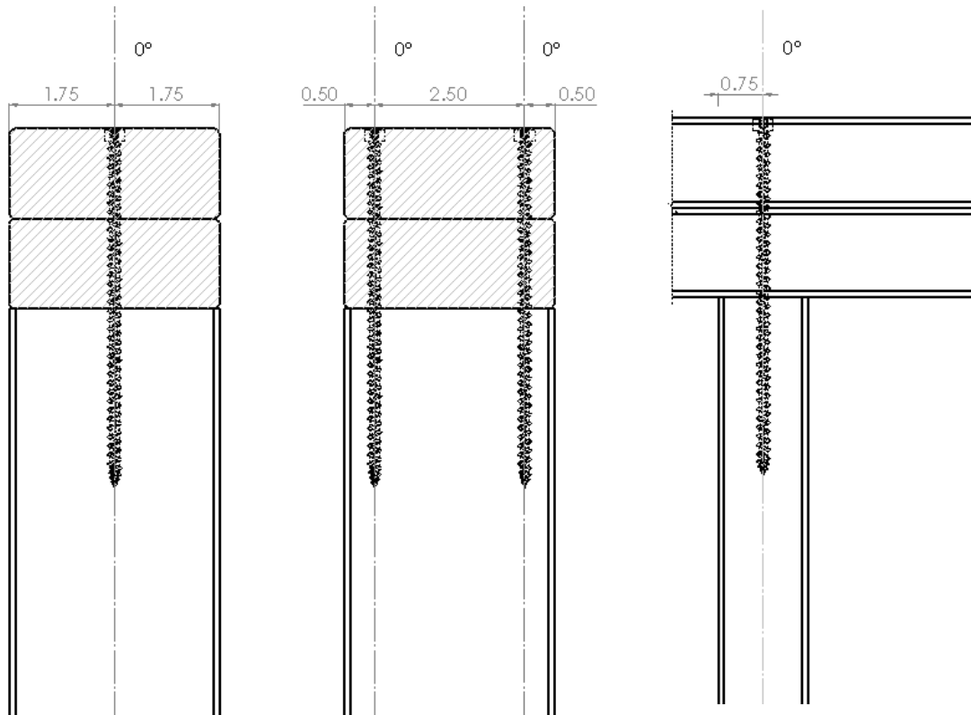
Figure 9. Stud to Top Plate – 0° (Perpendicular) Install Options
