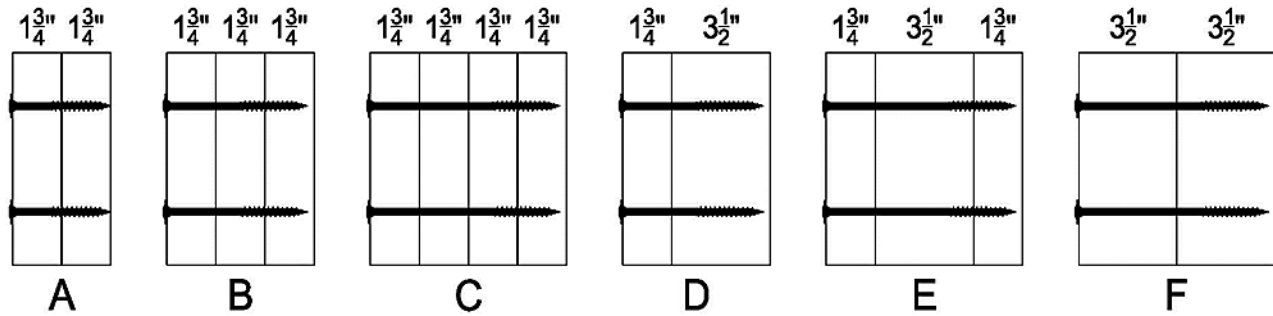
FIGURE 10. BIG TIMBER® SCREW SCL ASSEMBLES
