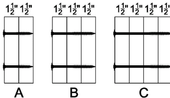
FIGURE 9. BIG TIMBER® SCREW SAWN LUMBER ASSEMBLIES
