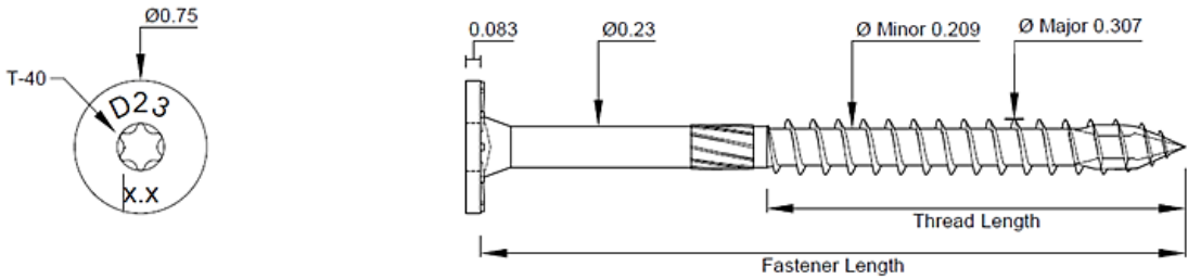
FIGURE 3. STARBORN® STRUCTURAL F23 SCREW (DIMENSIONS IN INCHES)
