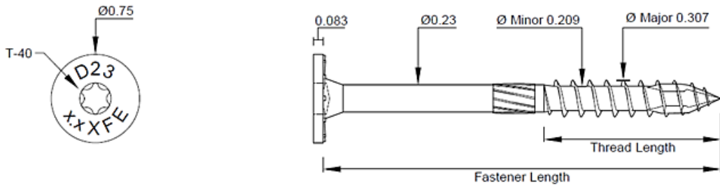
FIGURE 4. STARBORN® STRUCTURAL F23-E SCREW (DIMENSIONS IN INCHES)
