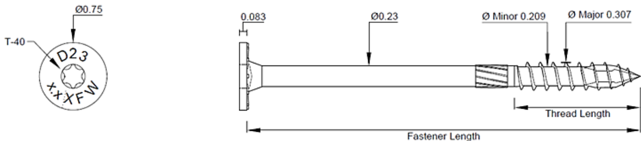
FIGURE 5. STARBORN® STRUCTURAL F23-W SCREW (DIMENSIONS IN INCHES)
