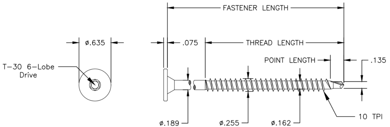
FIGURE 2. SIPLD FASTENER
