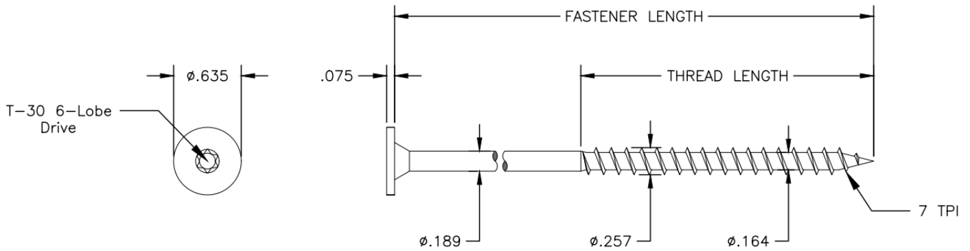
FIGURE 1. SIPTP FASTENER
