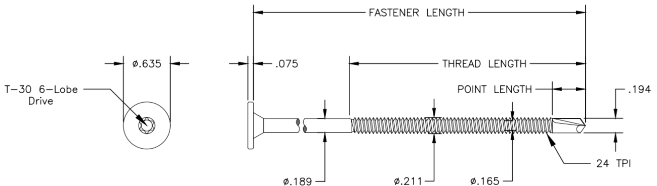
FIGURE 3. SIPHD FASTENER
