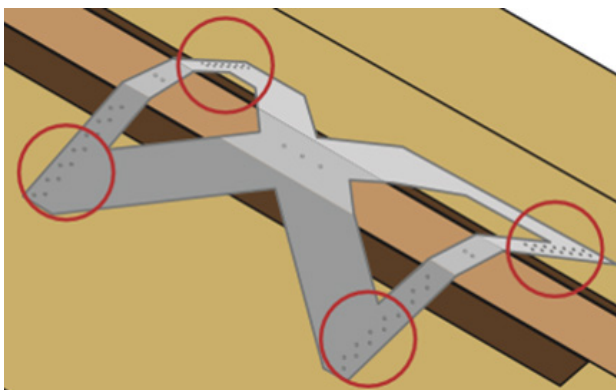
Figure 7. Shear-X™ Final Attachment
