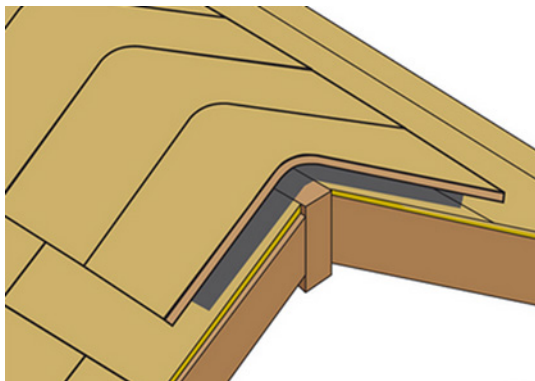
Figure 9. Ridge Cap Shingles Installed Post Shear-X™ Installation
