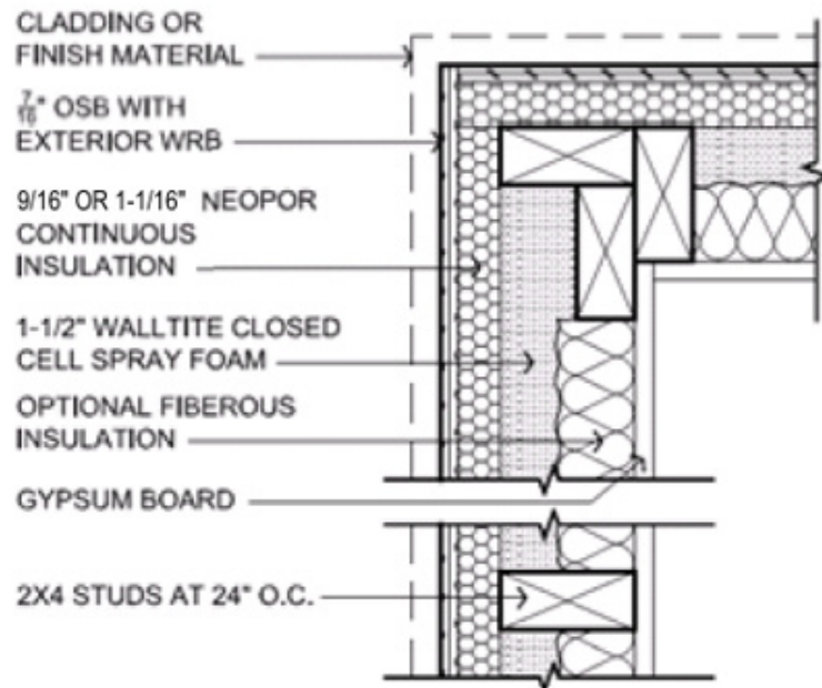
Figure 2. Cross Section of WALLTITE® HP+™ Wall X Series
