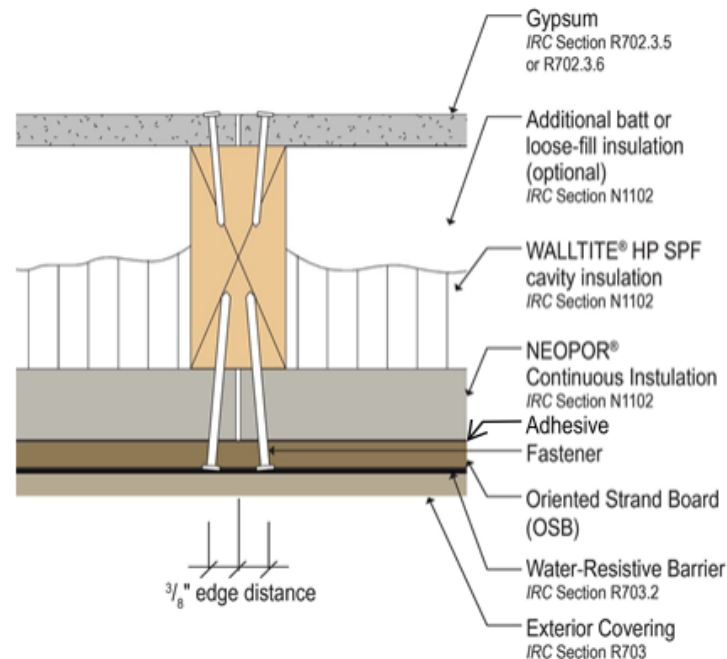
Figure 4. Fastening of Neopor®/OSB & Gypsum Sheathing
