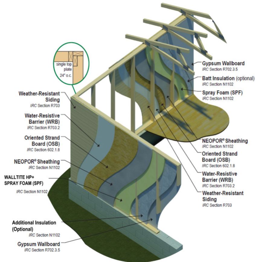
Figure 1. Illustration of BASF HP+™ Wall X Series System
