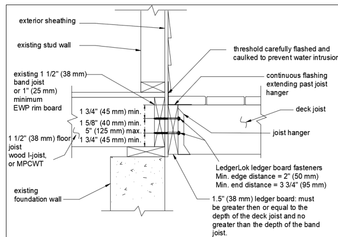
Figure 2. LedgerLOK Ledger Board Fasteners Deck Connection
