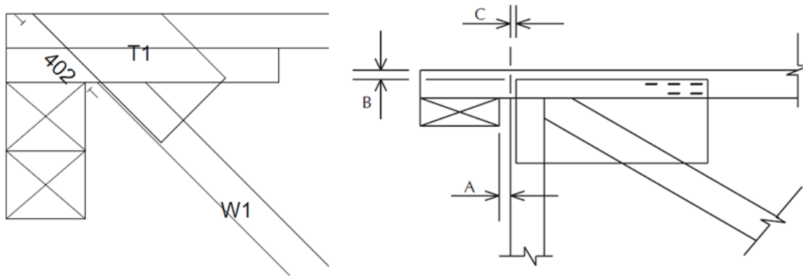
Figure 2. Trussway Alternative Bearing Detail (Left) and TPI 1 Figure 7.4-1(a) (Right)
