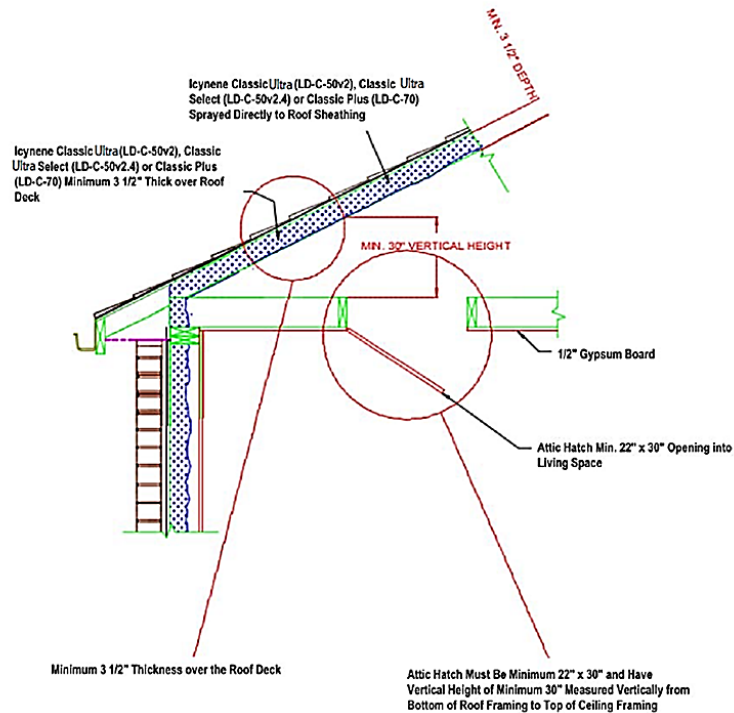
Figure 2. Classic Ultra, Classic Ultra Select and Classic Plus Used in an Unvented Attic Space
