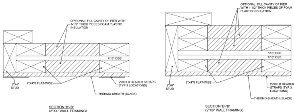
Figure 7. PFH Section B-B
