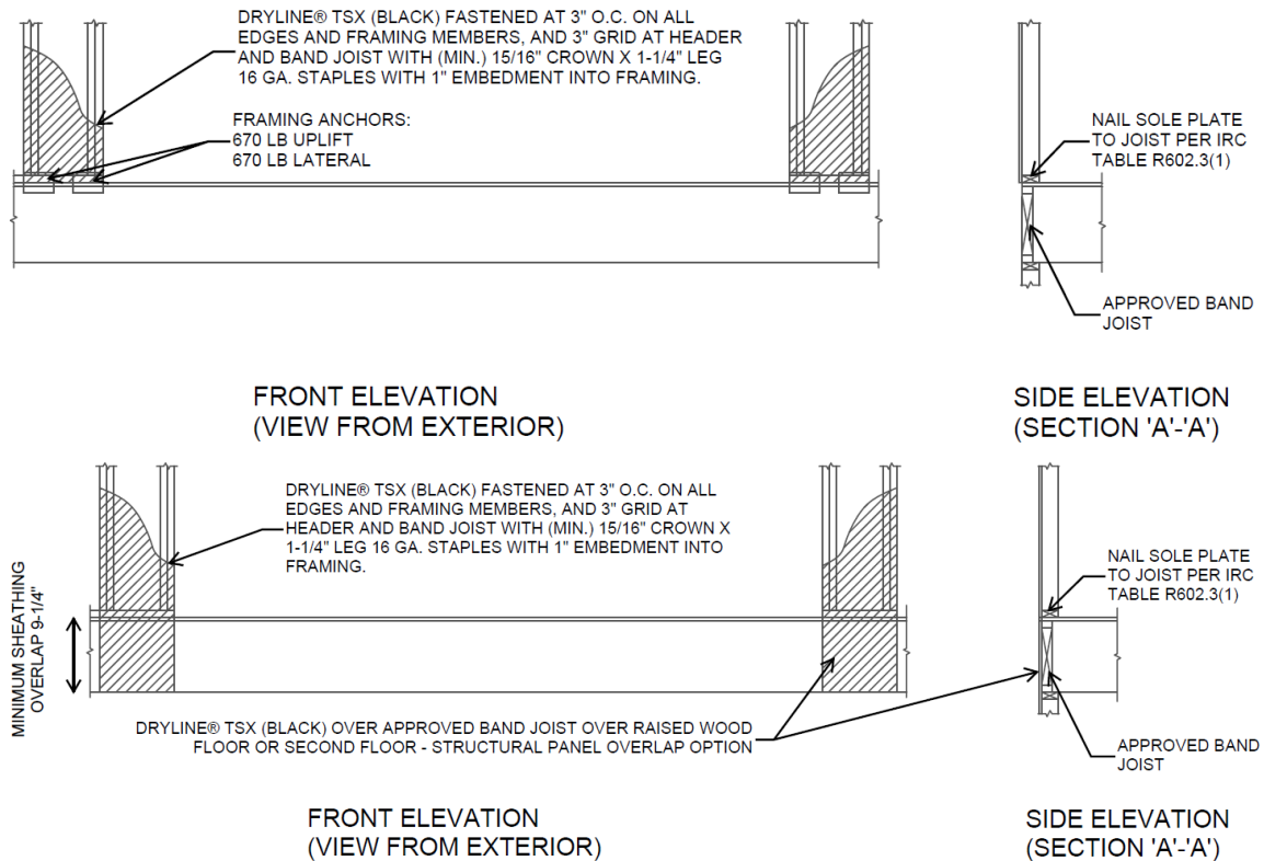
Figure 3. DRYline (Black) Structural Sheathing CS-PF – Anchorage Details
