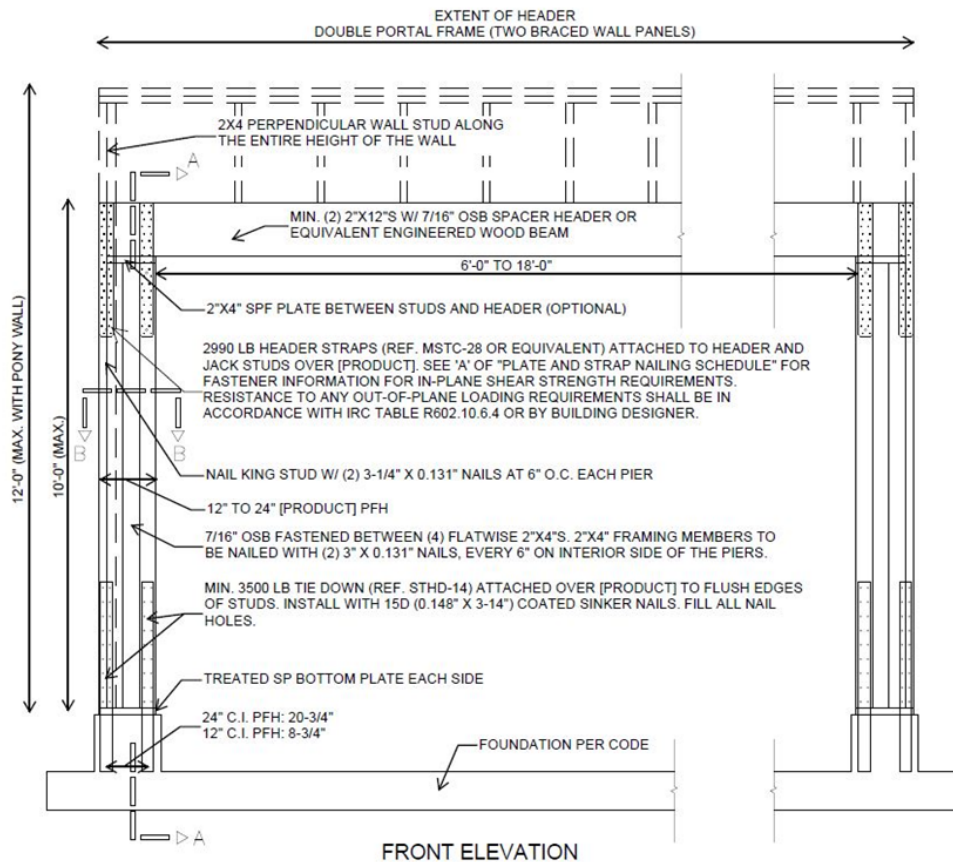
Figure 4. Construction Details of Thermo-Sheath (Black) 12" to 24" PFH
