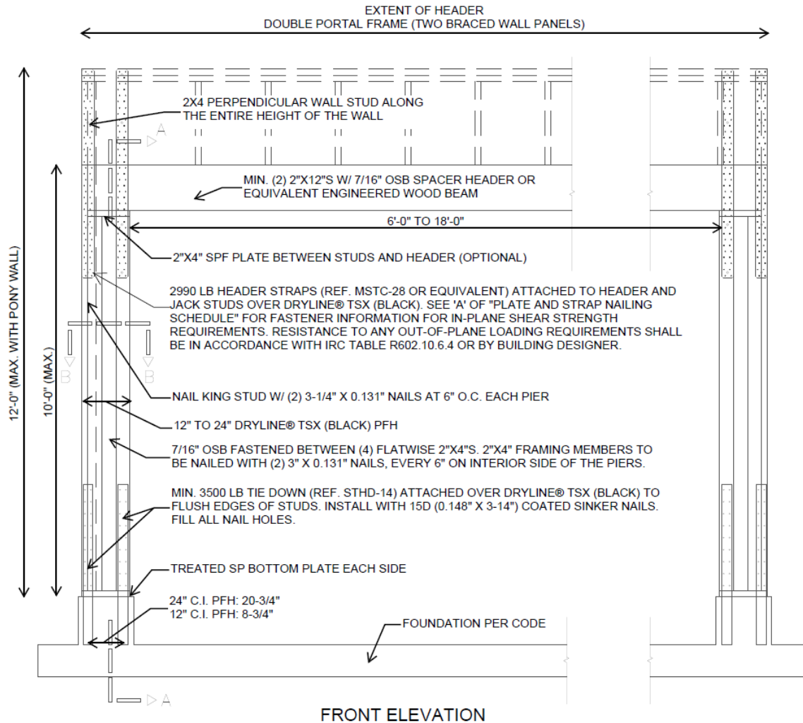
Figure 4. Construction Details of DRYline (Black) 12" to 24" PFH
