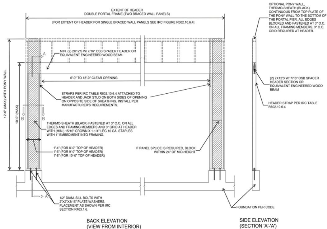
Figure 2. Thermo-Sheath (Black) Structural Sheathing CS-PF
