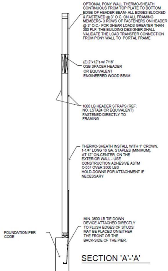
Figure 9. PFH Option 2 Section A-A
