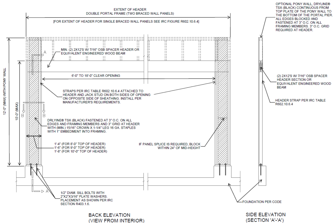
Figure 2. DRYline (Black) Structural Sheathing CS-PF
