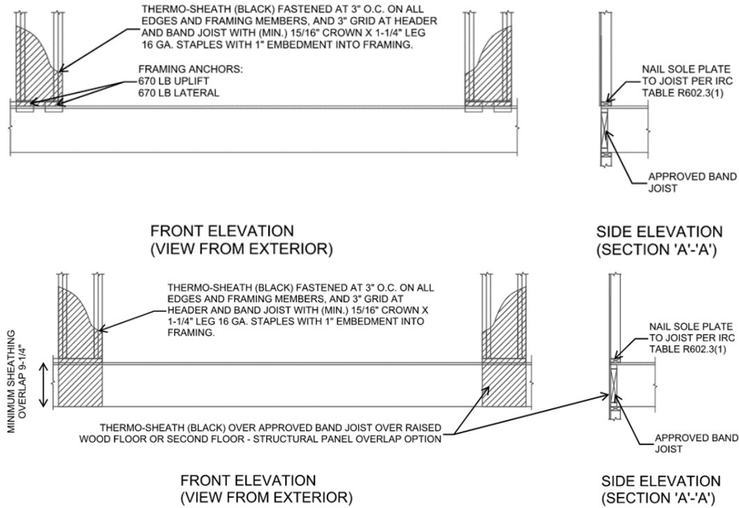
Figure 3. Thermo-Sheath (Black) Structural Sheathing CS-PF – Anchorage Details
