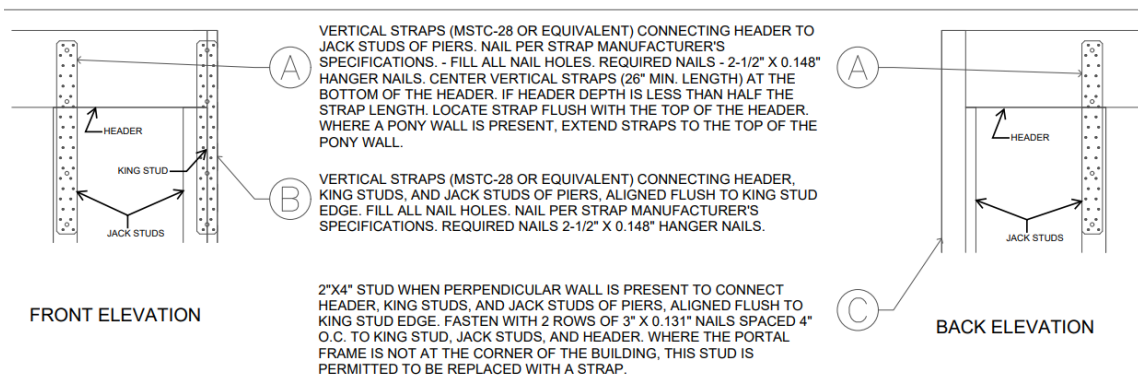
Figure 5. Header Connection Detail
