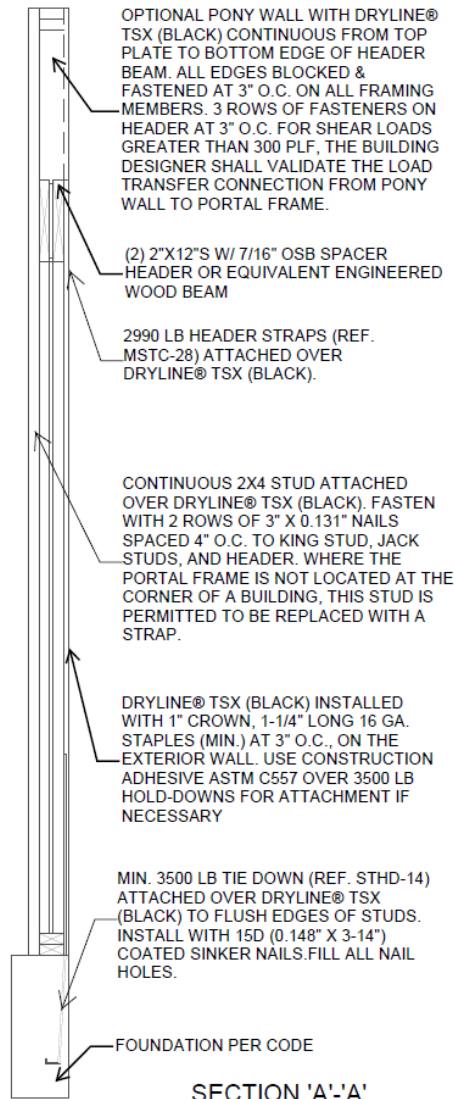
Figure 6. PFH Section A-A
