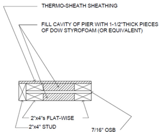
Figure 9. PFH Option 2 Section A-A
