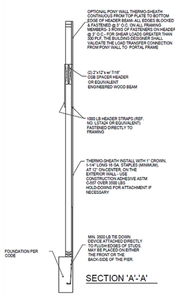
Figure 7. PFH Option 2 Section A-A
