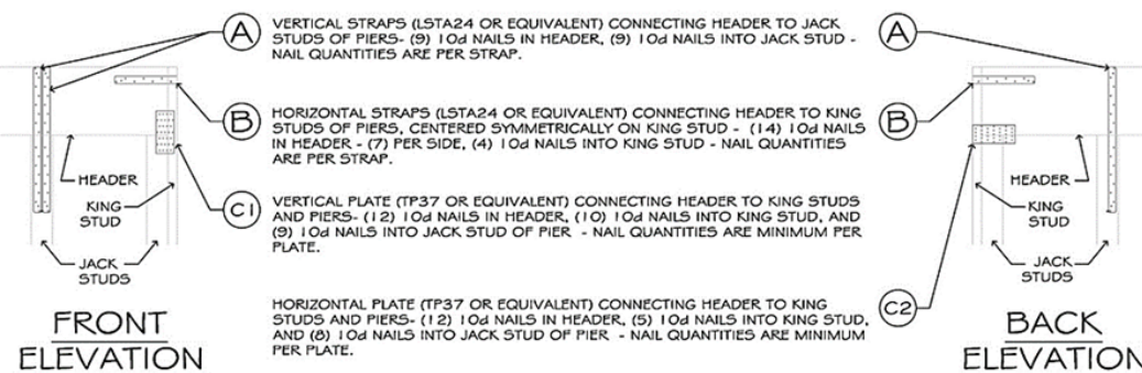
Figure 6. Construction Details of Thermo-Sheath (Green) 12" to 24" PFH – Option 2
