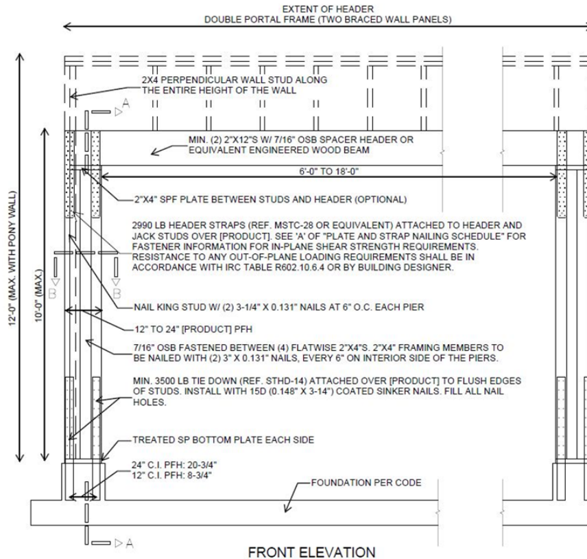
Figure 2. Construction Details of Thermo-Sheath (Green) 12" to 24" PFH – Option 1
