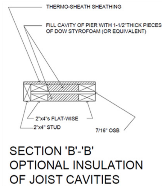
Figure 8. PFH Option 2 Section B-B
