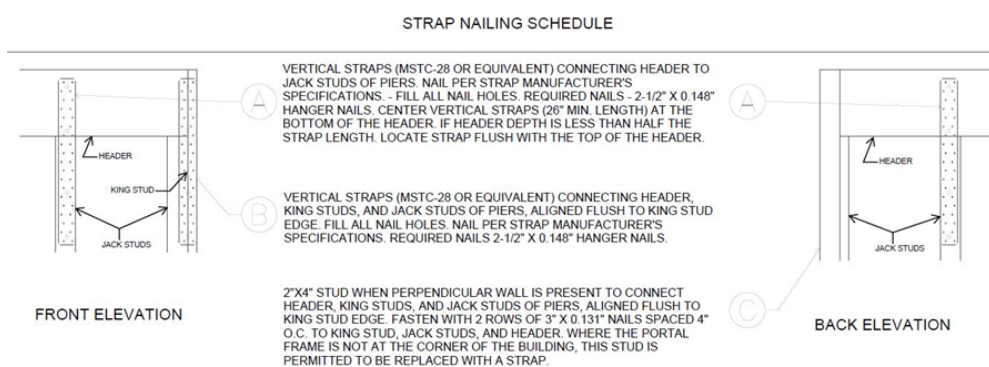
Figure 3. Header Connection Detail – Option 1
