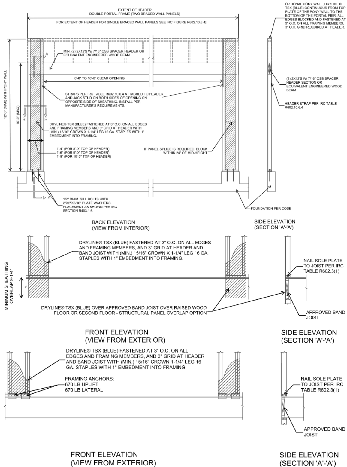
Figure 2. DRYline (Blue) Structural Sheathing CS-PF
