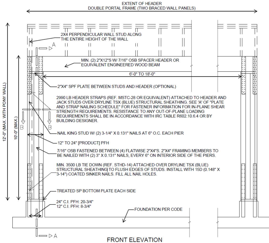
Figure 3. Construction Details of DRYline (Blue) Structural Sheathing 12" to 24" PFH – Option 1
