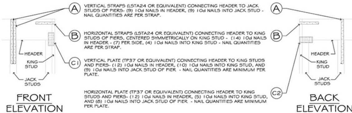
Figure 7. Construction Details of DRYline (Blue) Structural Sheathing 12" to 24" PFH – Option 2
