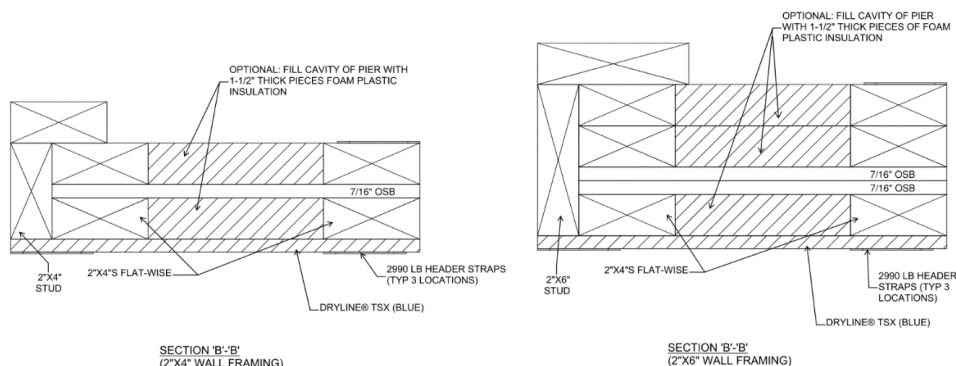
Figure 6. PFH Option 1 Section B-B
