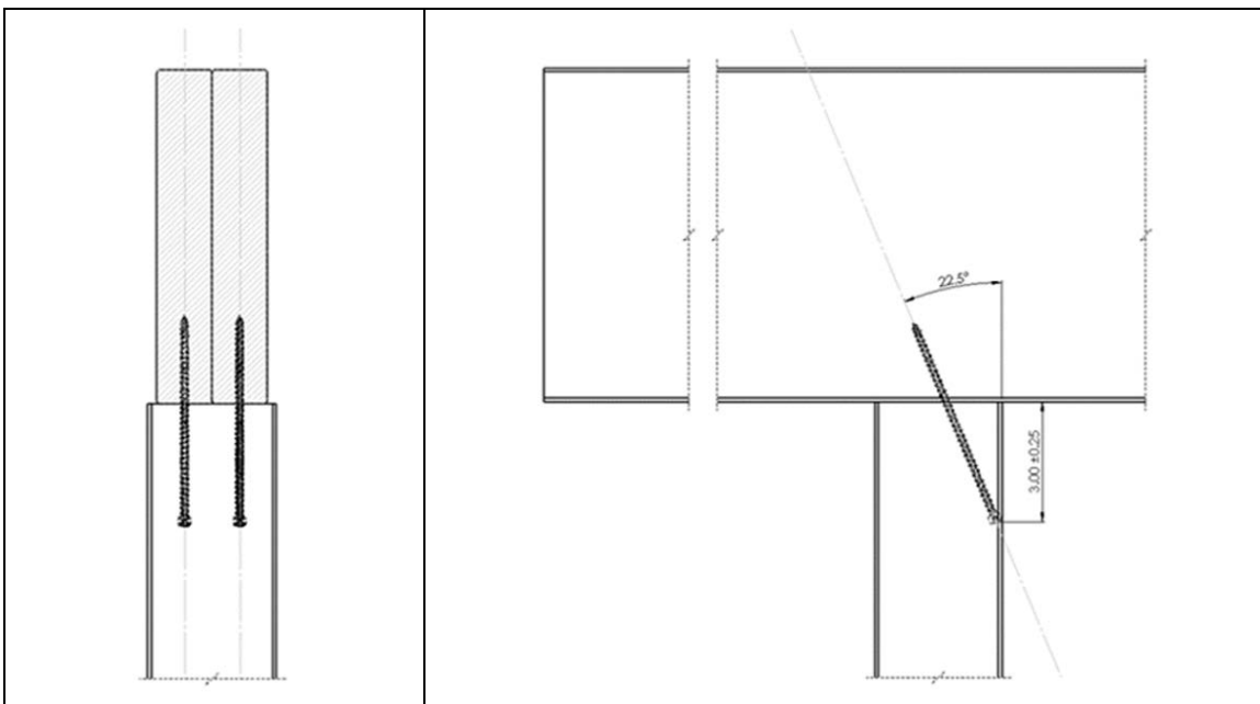
Figure 26. Post to 2-Ply Beam - Deck Connection, 2 Screws, 22.5°
