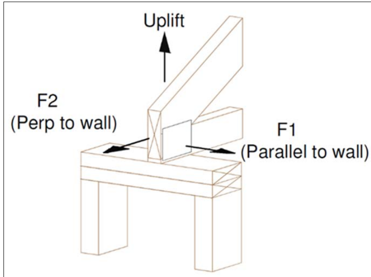
Figure 3. Uplift and Lateral Load Orientations
