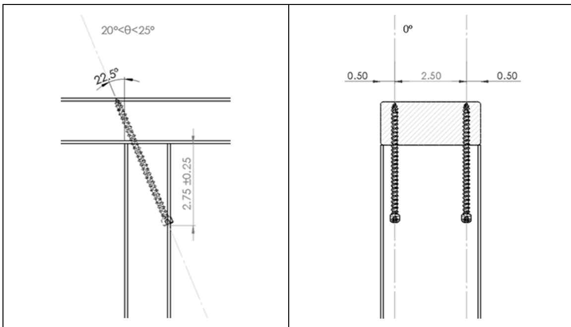
Figure 17. Stud to Top Plate – 22.5° (Angle), Two 4½" U2 Truss Screws Install Option
