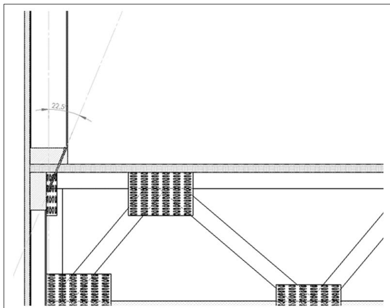
Figure 11. Installation of 4 1 / 2 " U2 Truss Screws at an Angle in Bottom Plate to Floor Truss/Joist Applications
