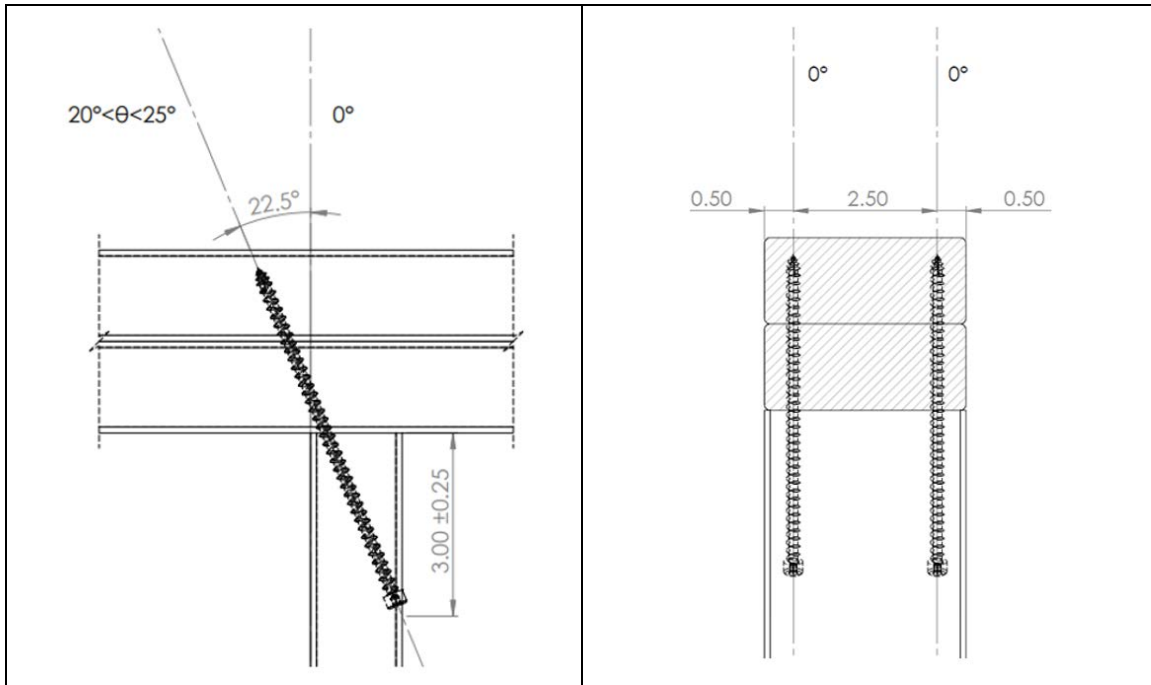
Figure 14. Stud to Top Plate – 22.5° (Angle), Two 6" U2 Truss Screws Install Option
