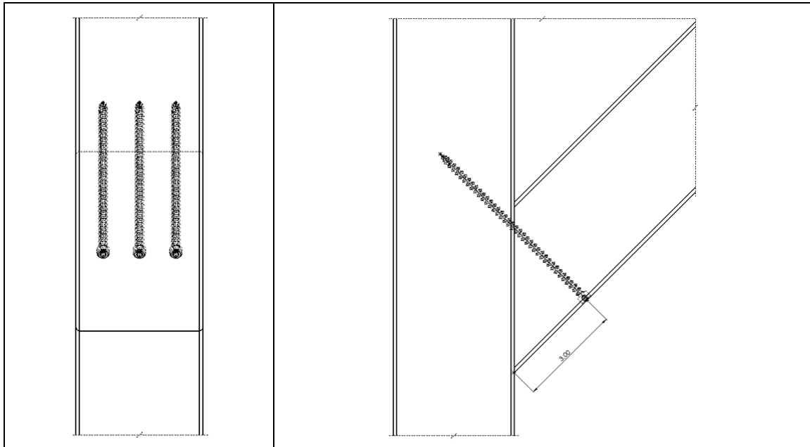
Figure 29. 4 x 4 Diagonal Brace Connection using 6" U2 Truss Screws
