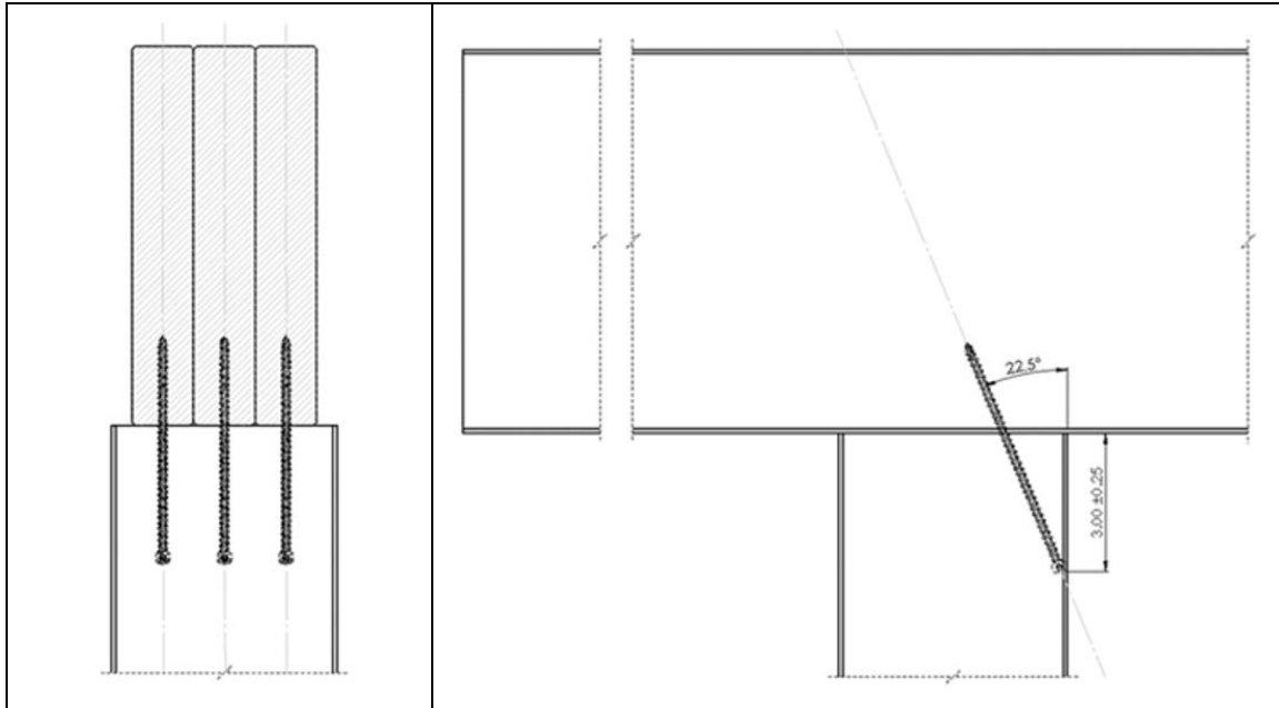
Figure 27. Post to 3-Ply Beam - Deck Connection
