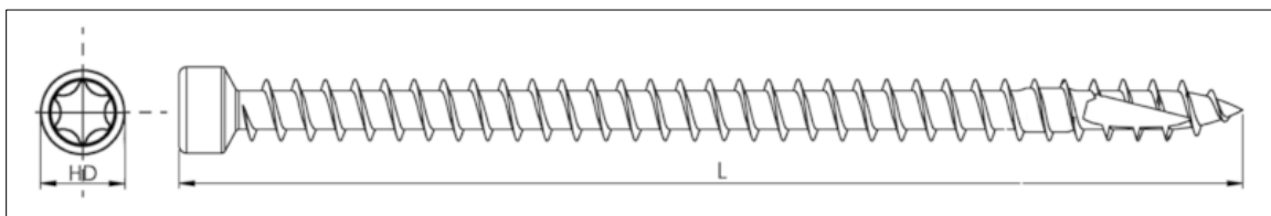
Figure 1. U2 Truss Screw
