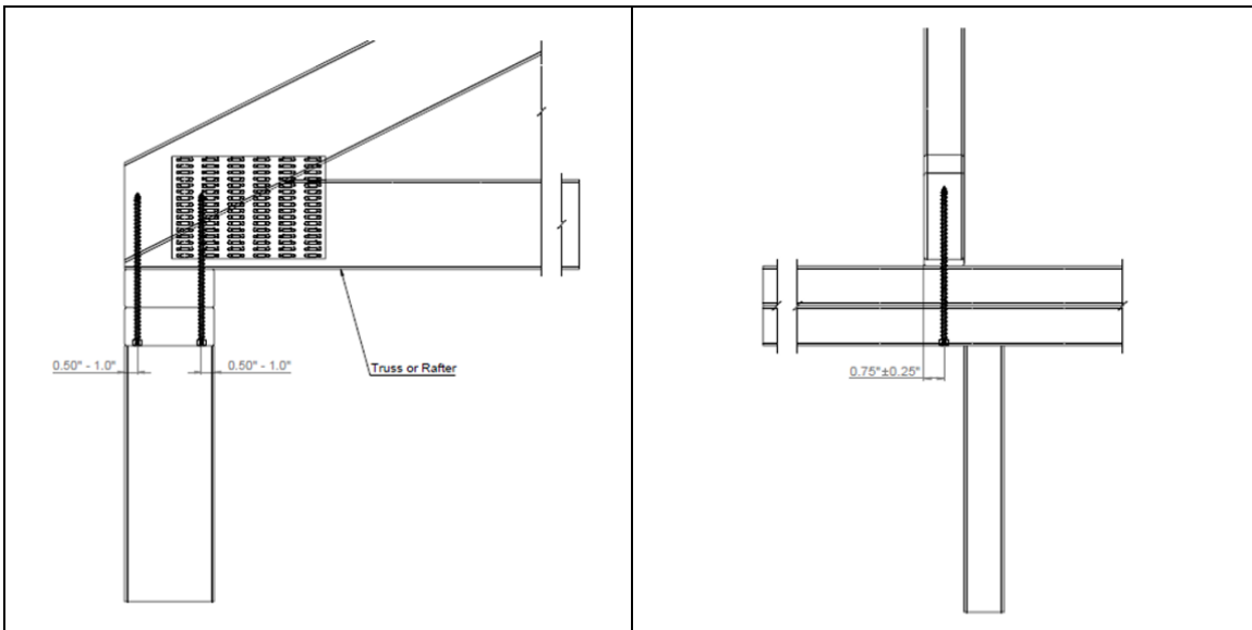
Figure 6. Installation of Two U2 Truss Screws in Truss to Top Plate Connection – Perpendicular
