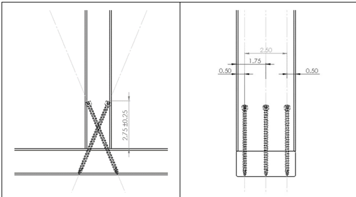
Figure 21. Stud to Bottom Plate – 22.5° (Angle), Three 4½" U2 Truss Screws Install Option
