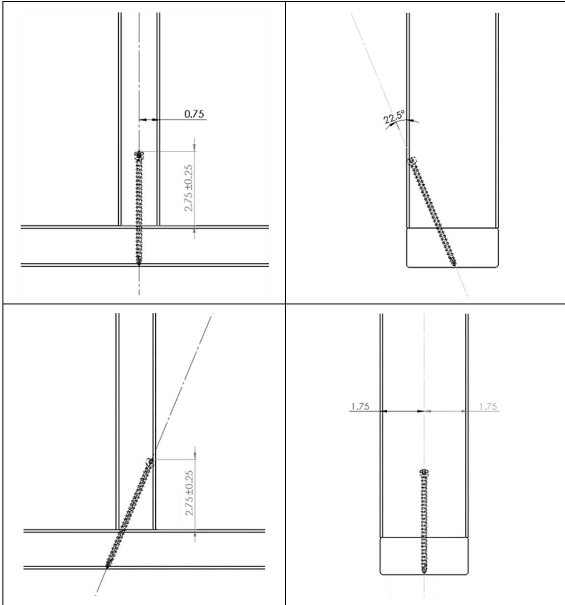
Figure 19. Stud to Bottom Plate – 22.5° (Angle), One 4½" U2 Truss Screw Option
