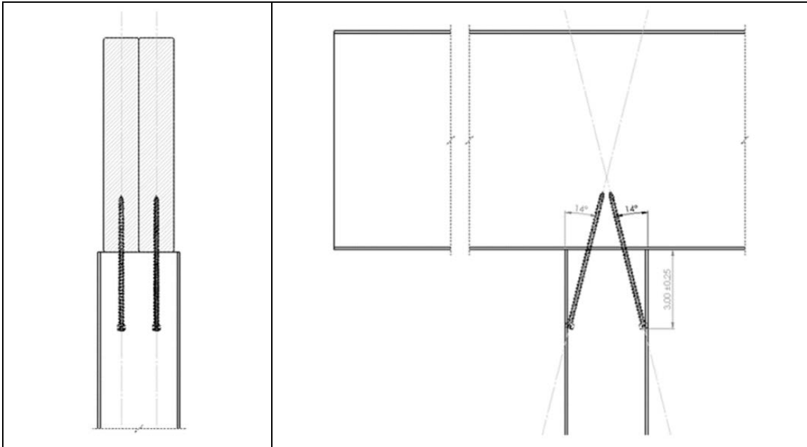
Figure 25. Post to 2-Ply Beam - Deck Connection, 4 Screws, 14°
