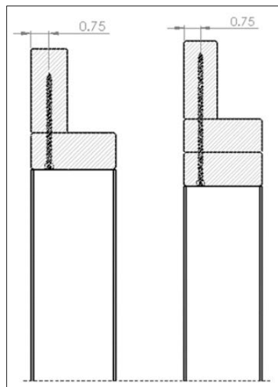
Figure 8. Gable End Truss to Top Plate Installation Configuration
