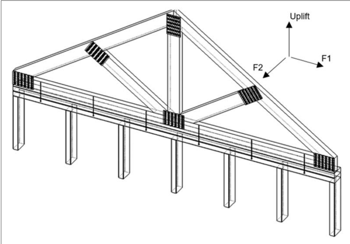
Figure 7. Gable End Truss to Top Plate - Uplift and Lateral Load (F1 and F2) Directions
