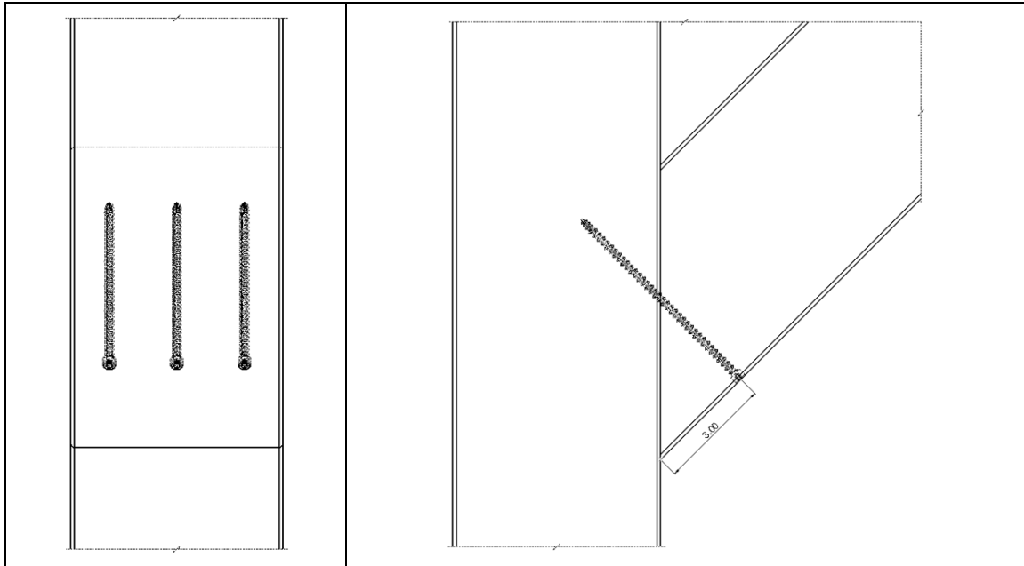
Figure 30. 6 x 6 Diagonal Brace Connection using 6" U2 Truss Screws
