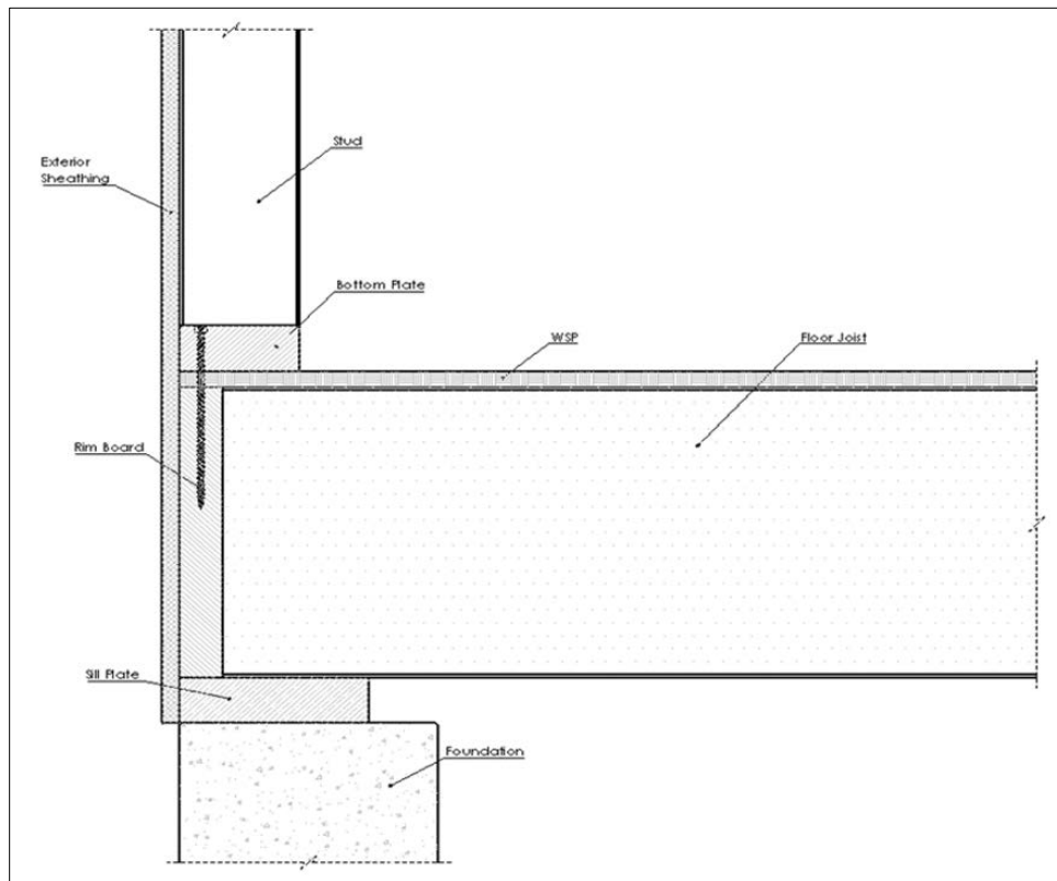
Figure 23. Fastener in Bottom Plate to Rim Board Connection
