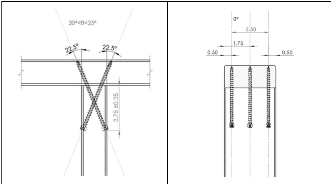
Figure 18. Stud to Top Plate – 22.5° (Angle), Three 4½" U2 Truss Screws Install Option
