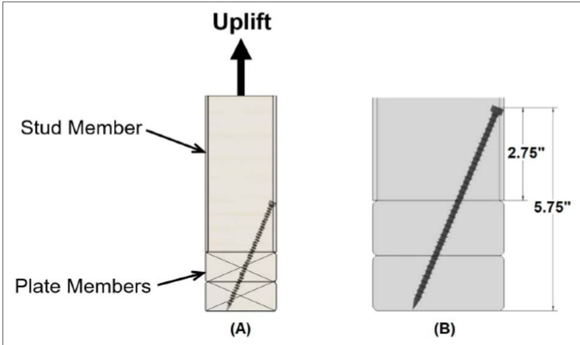
Figure 22. Stud to Double Bottom Plate – 22.5° (Angle), One 6" U2 Truss Screw Option
