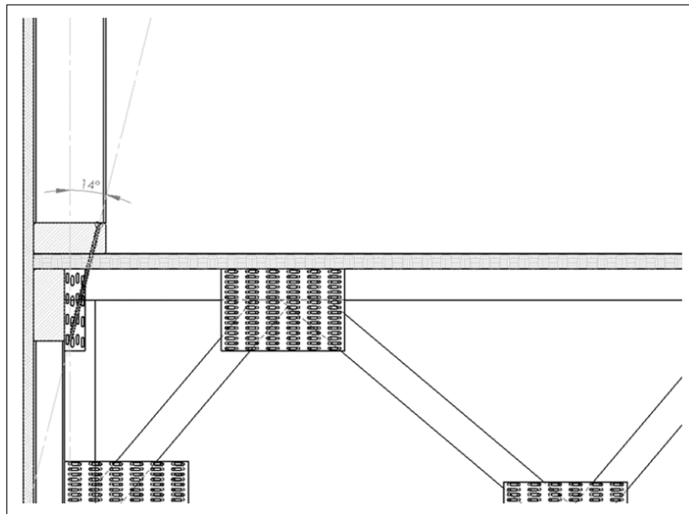
Figure 10. Installation of 6" U2 Truss Screws at an Angle in Bottom Plate to Floor Truss/Joist Applications
