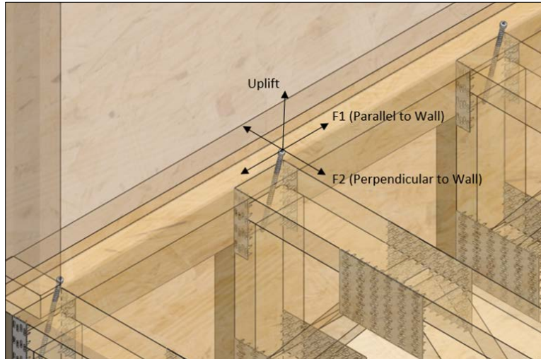
Figure 9. Uplift and (F1 and F2) Load Directions
