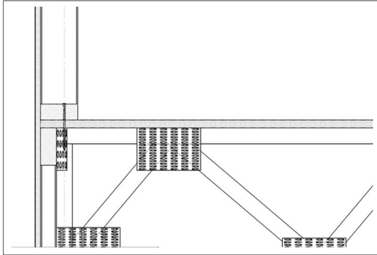
Figure 12. Perpendicular Installation of 4 \frac{1}{2} " U2 Truss Screws in Bottom Plate to Floor Truss/Joist Applications
