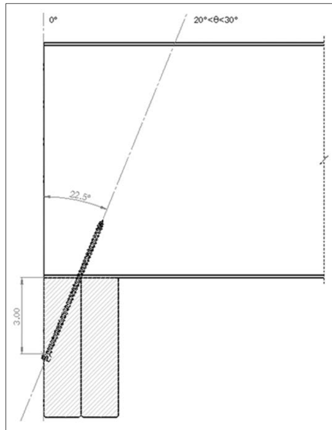
Figure 24. Joist to Beam - Deck Connection
