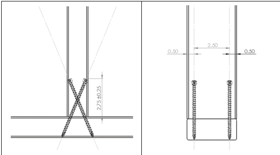
Figure 20. Stud to Bottom Plate – 22.5° (Angle), Two 4½" U2 Truss Screws Install Option
