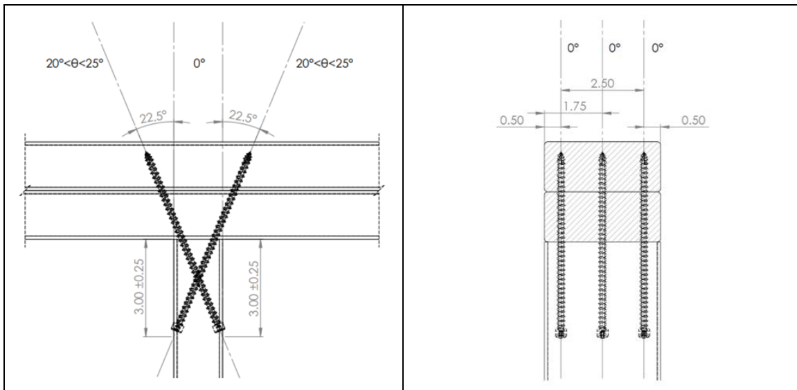
Figure 15. Stud to Top Plate – 22.5° (Angle), Three 6" U2 Truss Screws Install Option
