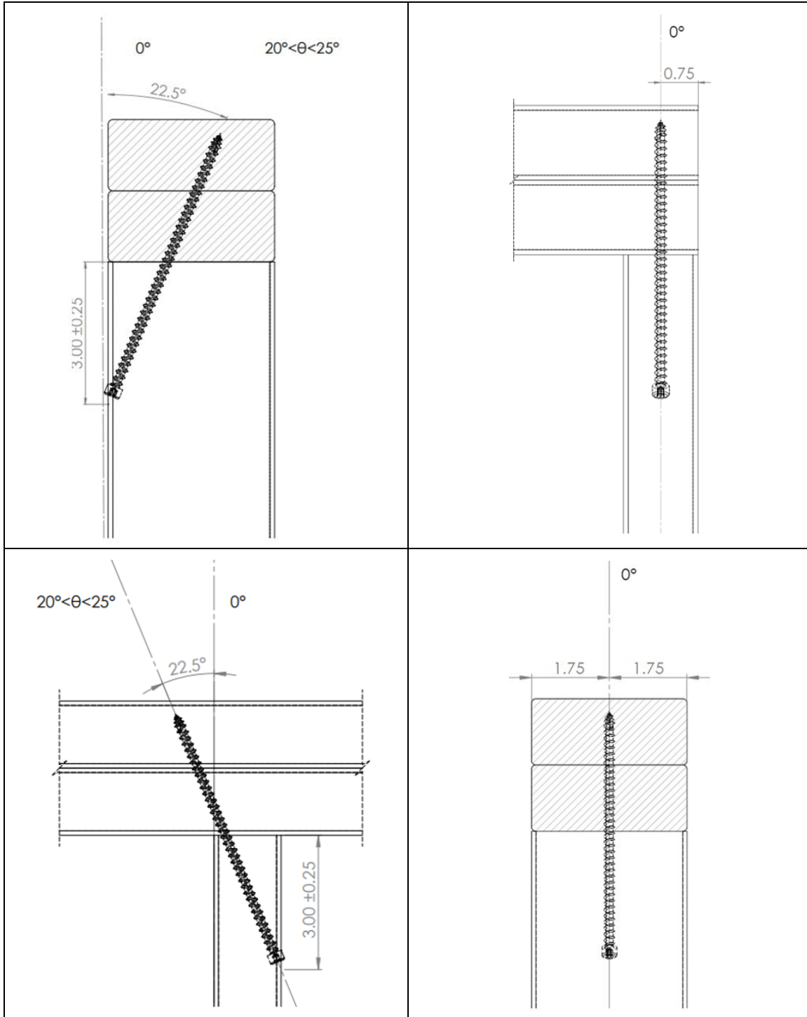
Figure 13. Stud to Top Plate – 22.5° (Angle), One 6" U2 Truss Screw Options
