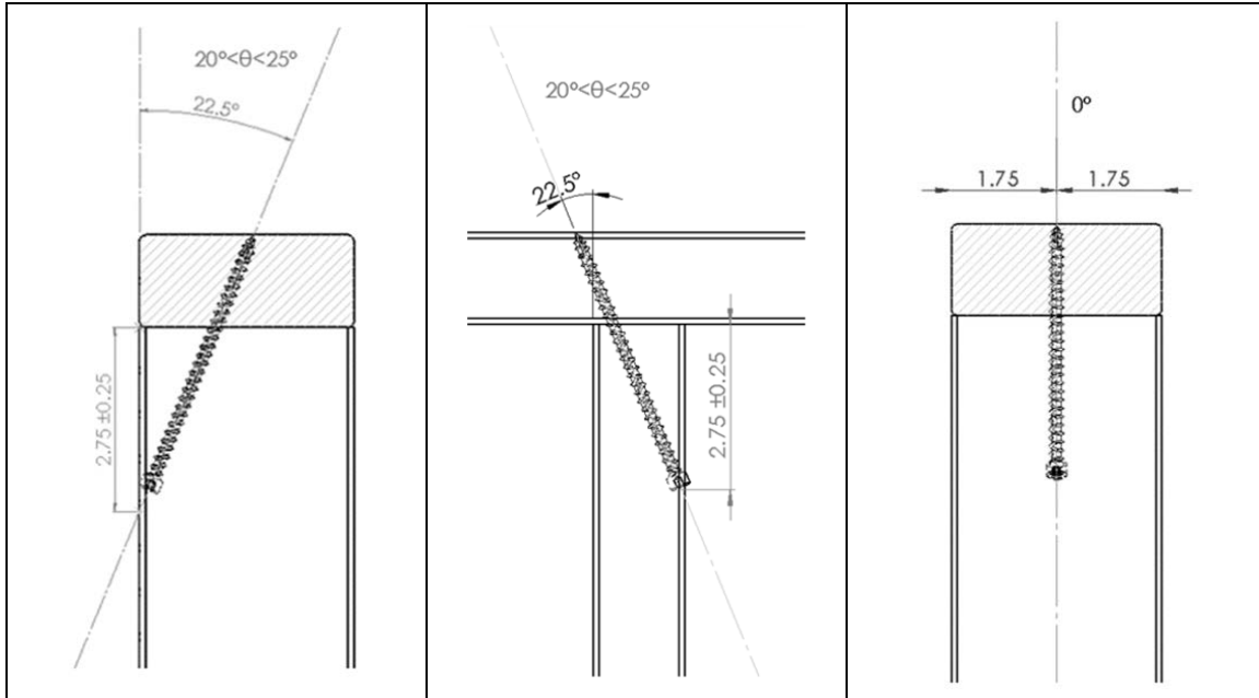
Figure 16. Stud to Top Plate – 22.5° (Angle), One 4½" U2 Truss Screw Options
