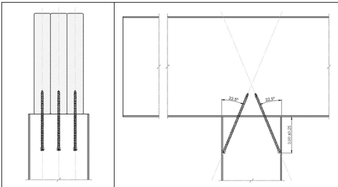
Figure 28. Post to 3-Ply Beam - Deck Connection
