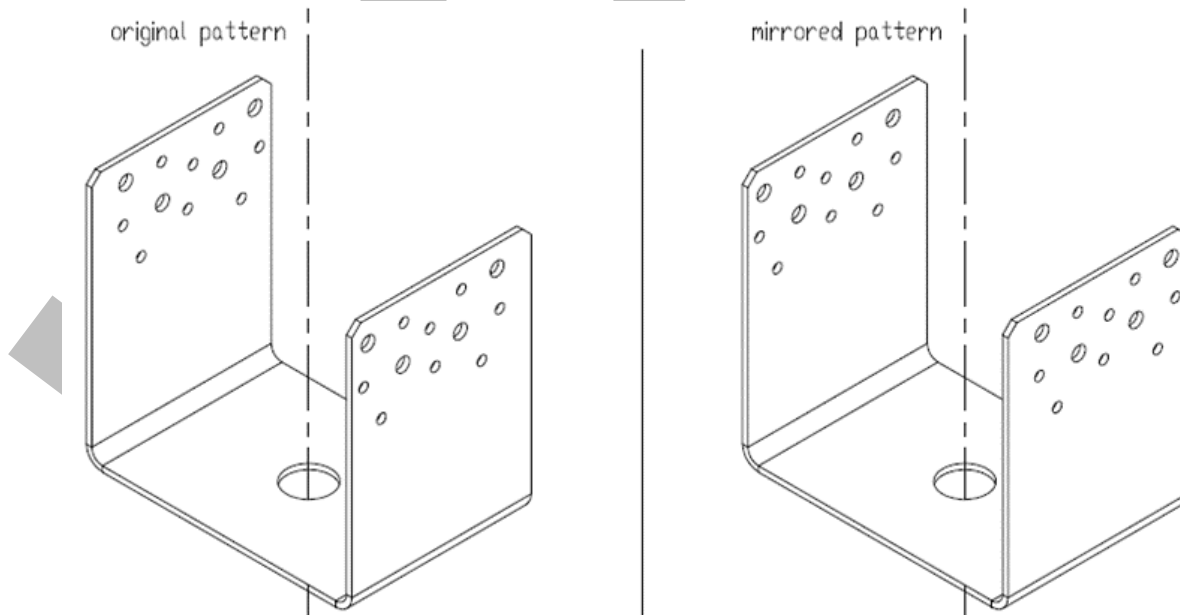
Figure 5. U-Plate Top Plate Variants
