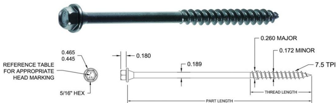
Figure 1. TimberLOK Fastener
