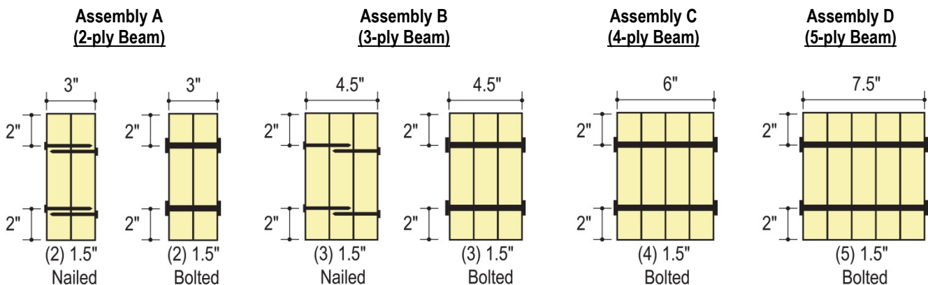
Figure 1. Connection Requirements for Multiple Member Side-Loaded Beams
