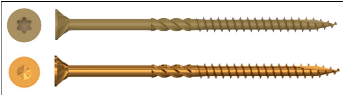
Figure 6. #10 Product 1 - CSH-TP TC Fastener with Exterior Coating (Top) and Interior Coating (Bottom)
