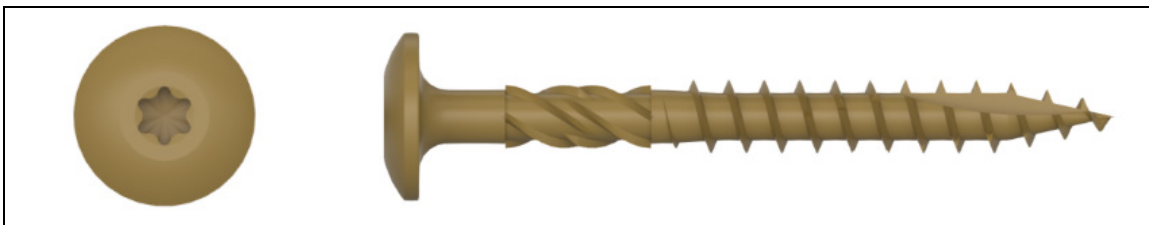
Figure 7. #10 Grip Fast Premium Cabinet Screws
