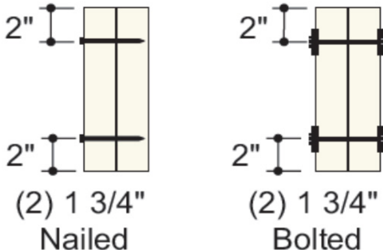
Figure 1. Assembly A (2-Ply Beam)
