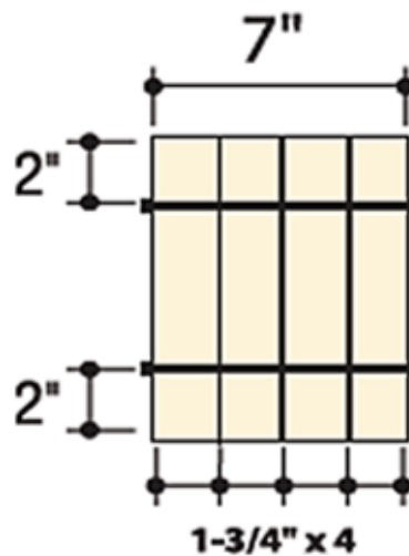
Figure 3. Assembly C (4-Ply Beam)
