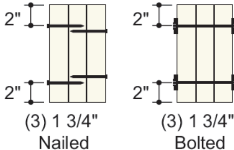
Figure 2. Assembly B (3-Ply Beam)
