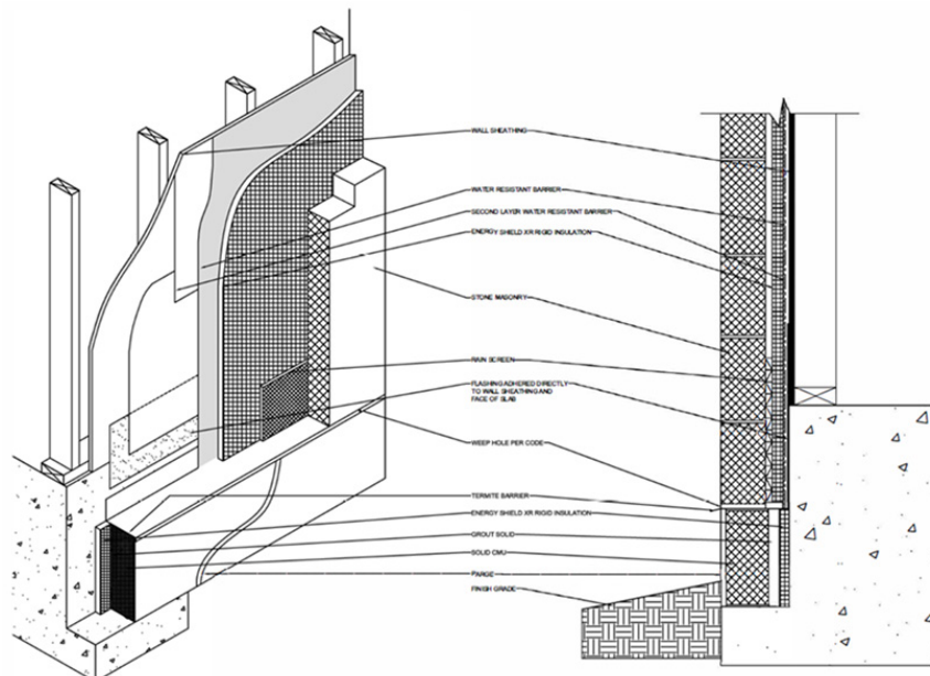
Figure 4. Stone Masonry Vener
