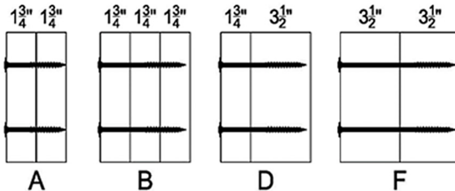
Figure 3. SCL Assembly Configurations
