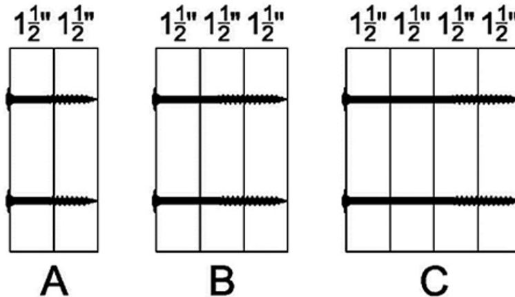
Figure 2. Sawn Lumber Assembly Configuration
