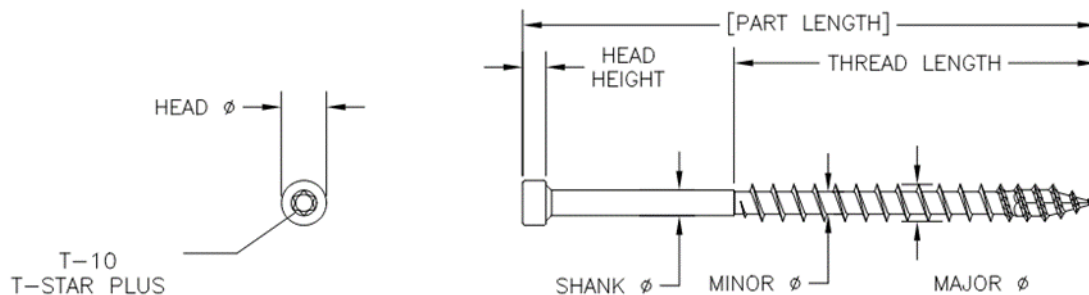
Figure 1. SPAX #8 (XTT-08) PowerTrim Screw
