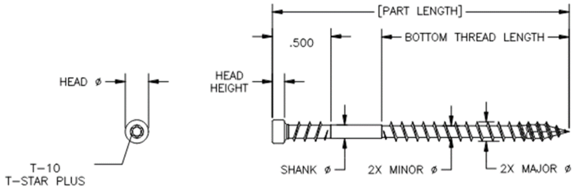
Figure 2. SPAX #8 (XTT-08D) PowerTrim Screw
