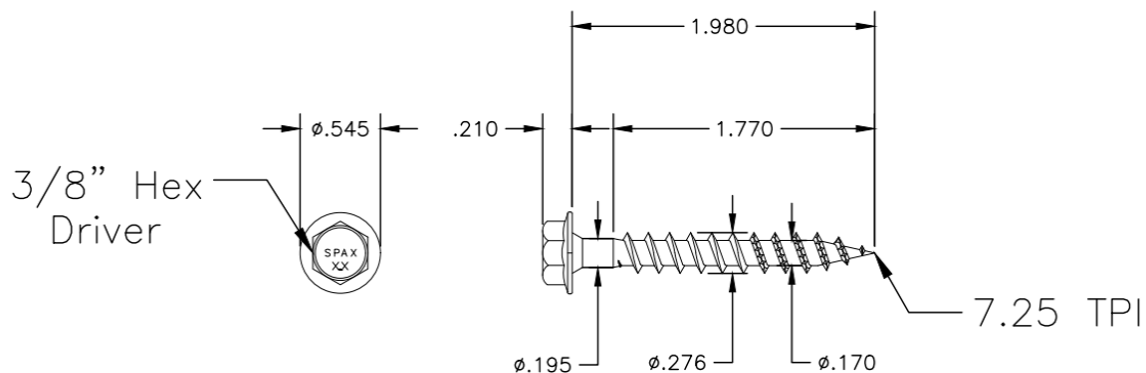
Figure 1. XH250-2000 Fastener
