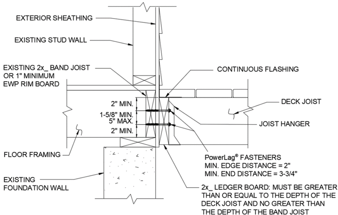
Figure 2. SPAX PowerLags Fasteners Deck Connection
