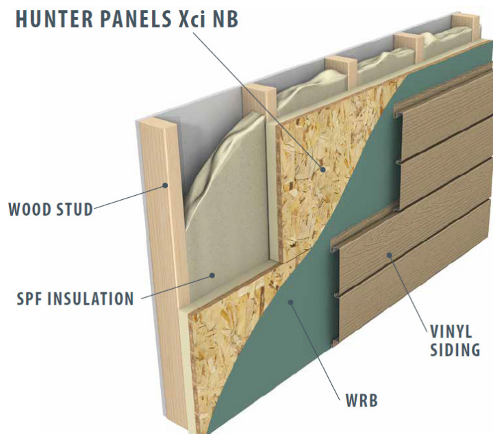
Figure 1. Xci NB with SPF Insulation
