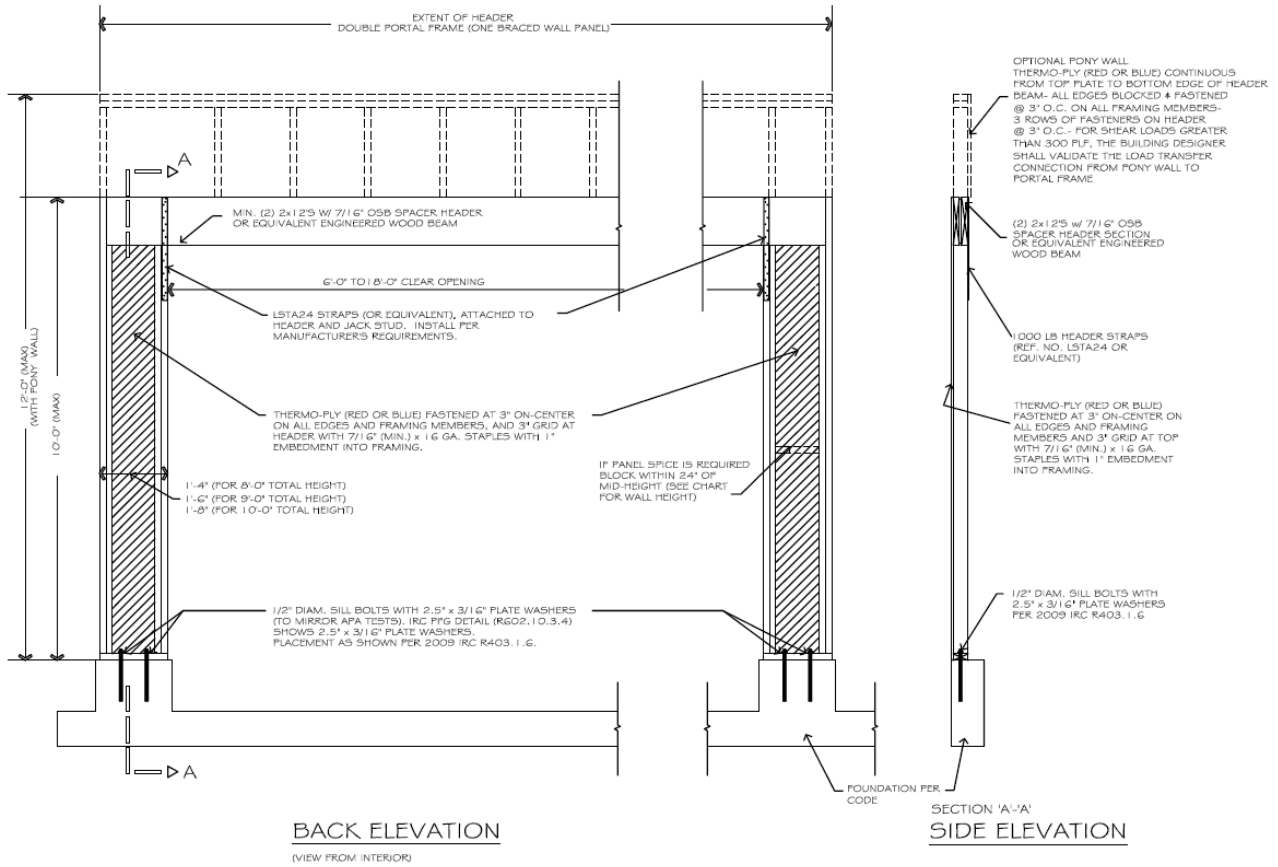
Figure 2: Thermo-Ply® Blue Structural Sheathing CS-PF Back Elevation
