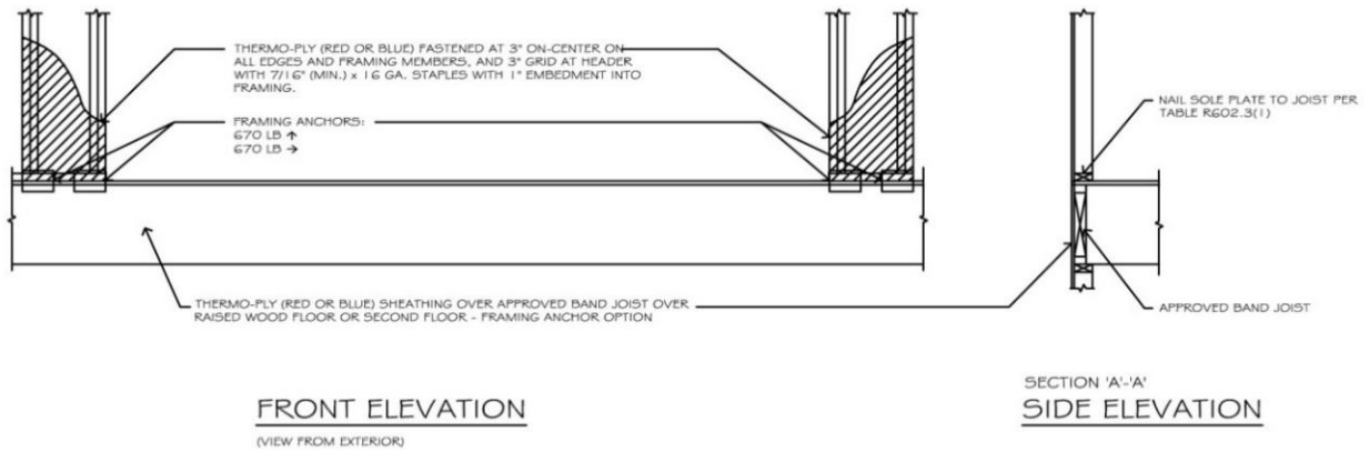
Figure 3: Thermo-Ply® Blue Structural Sheathing CS-PF Front Elevation 1
