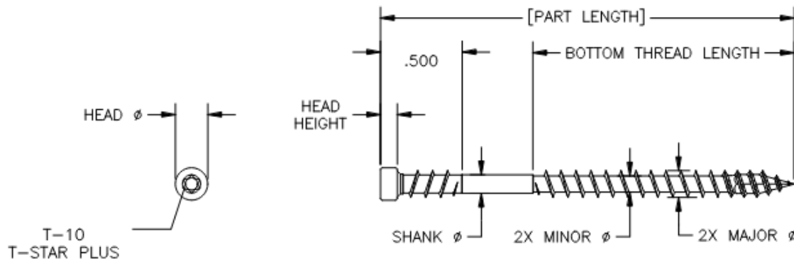
Figure 2. SPAX® XTT08D Fastener
