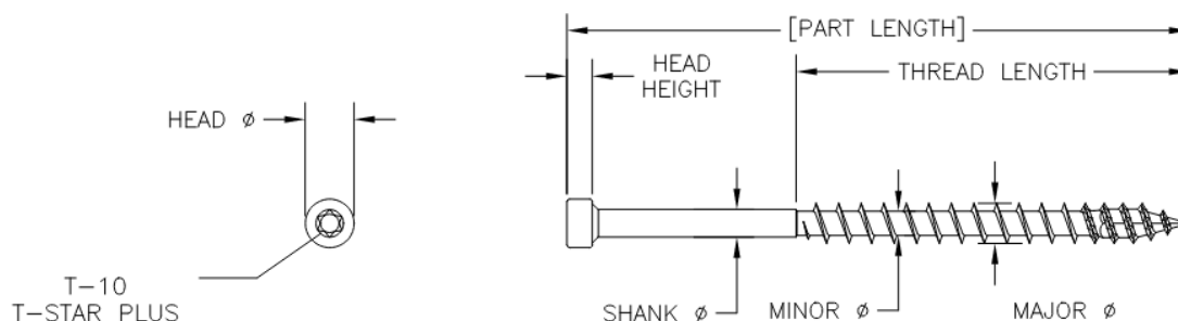
Figure 1. SPAX® XTT08 Fastener
