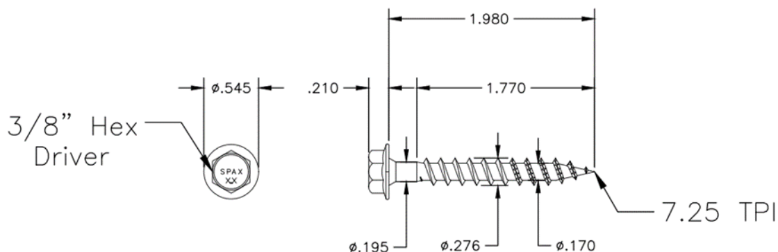
Figure 1. XH250-2000 Fastener
